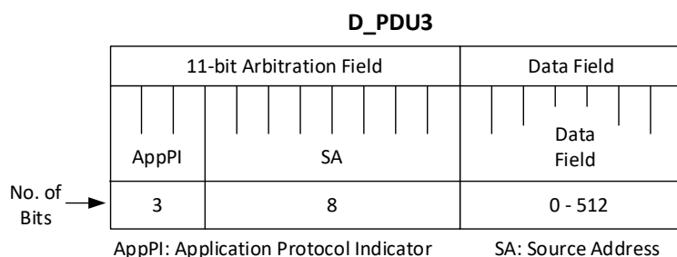
Figure 5 - D_PDU formats
