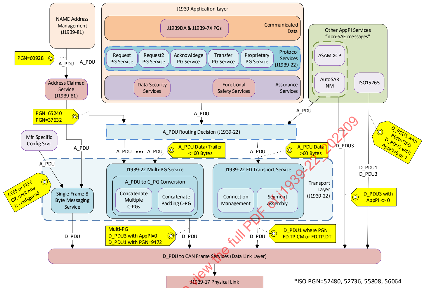
Figure 2 - Transmit model
