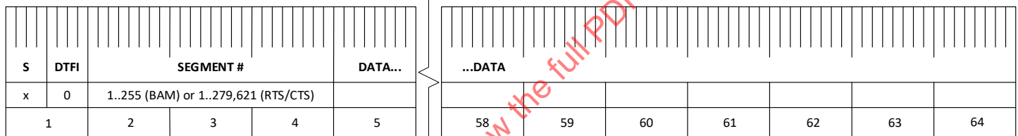
Figure 38 - FD transport protocol - data transfer message
