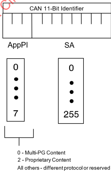
Figure 8 - D_PDU3 format
