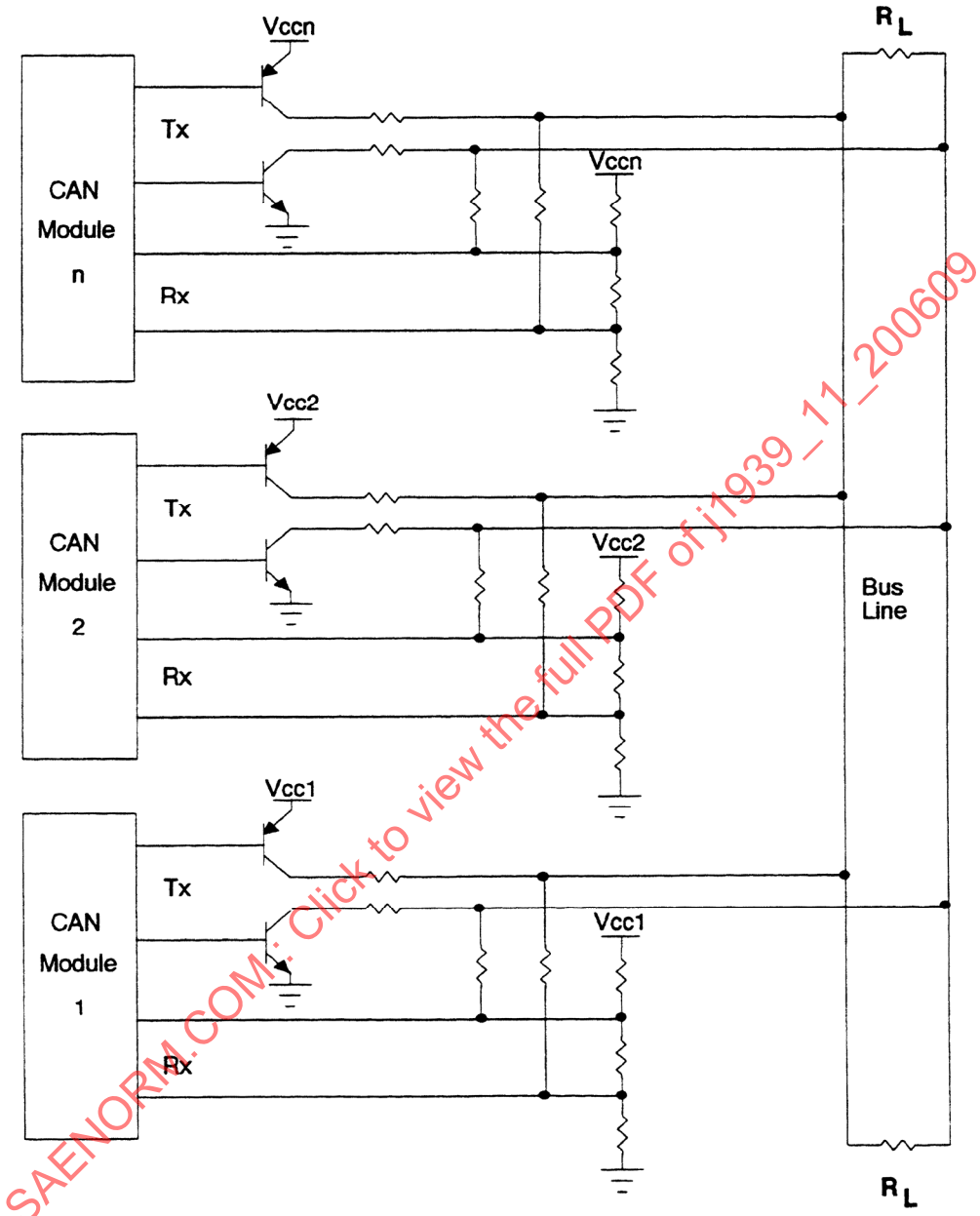
FIGURE 2—PHYSICAL LAYER FUNCTIONAL
