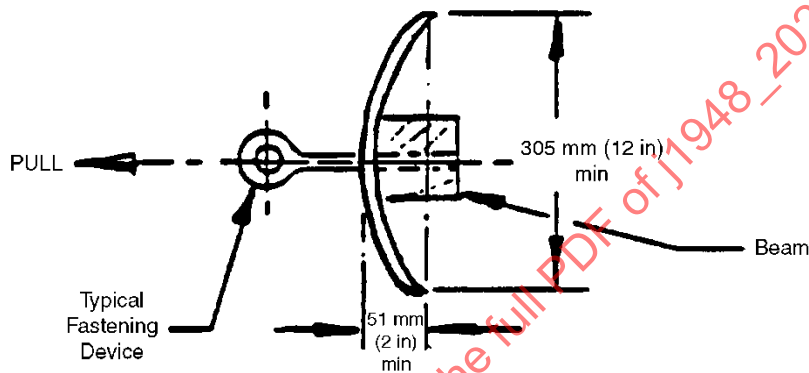
FIGURE 1 - END VIEW BODY BLOCK
