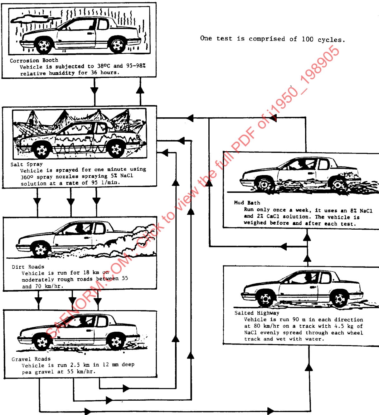
FIGURE 7—AMERICAN MOTORS CORPORATION VEHICLE CORROSION TESTING
