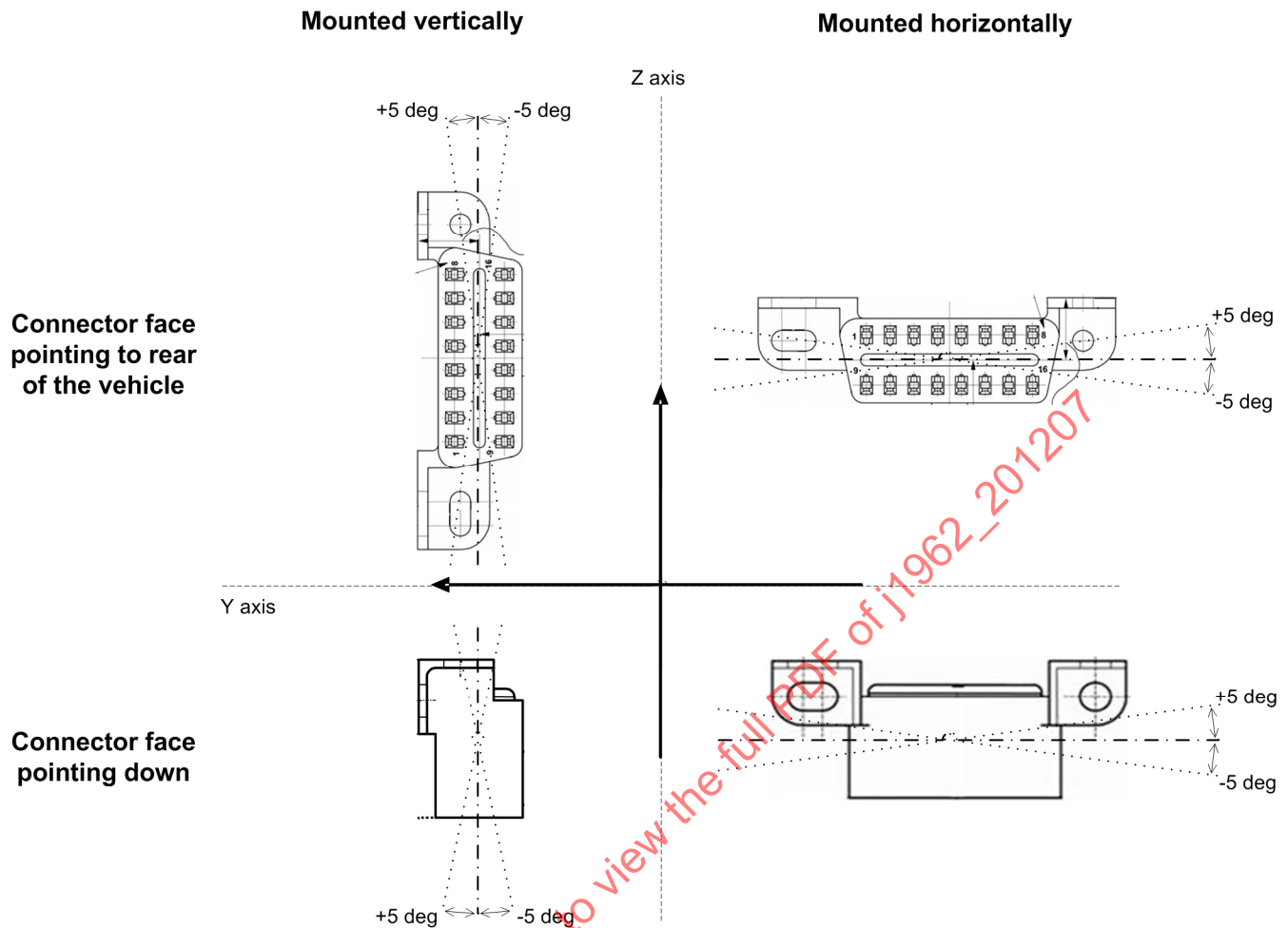
FIGURE 2 – CONNECTOR OREINTATION (MOUNTING LIMITS)
