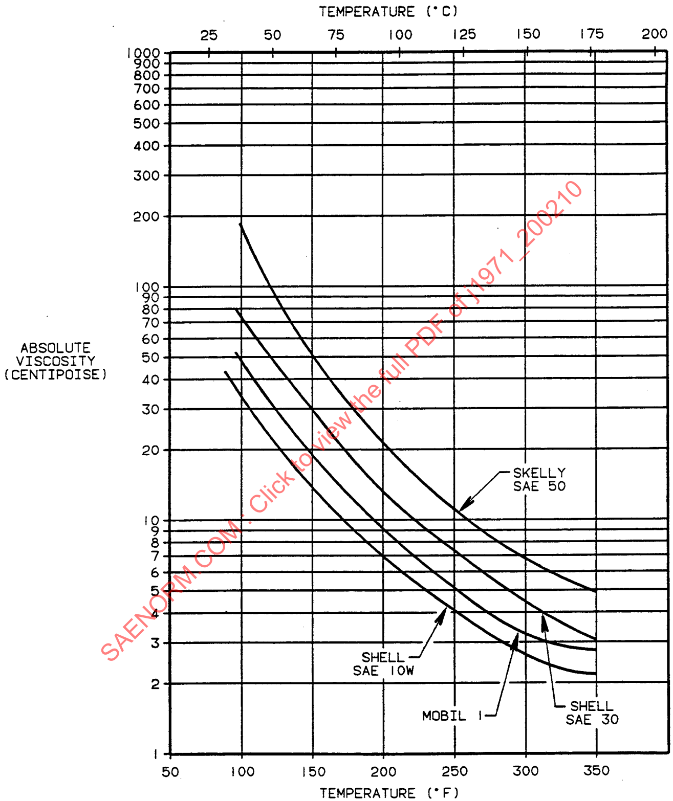
FIGURE 6—ABSOLUTE OIL VISCOSITY VERSUS TEMPERATURE
