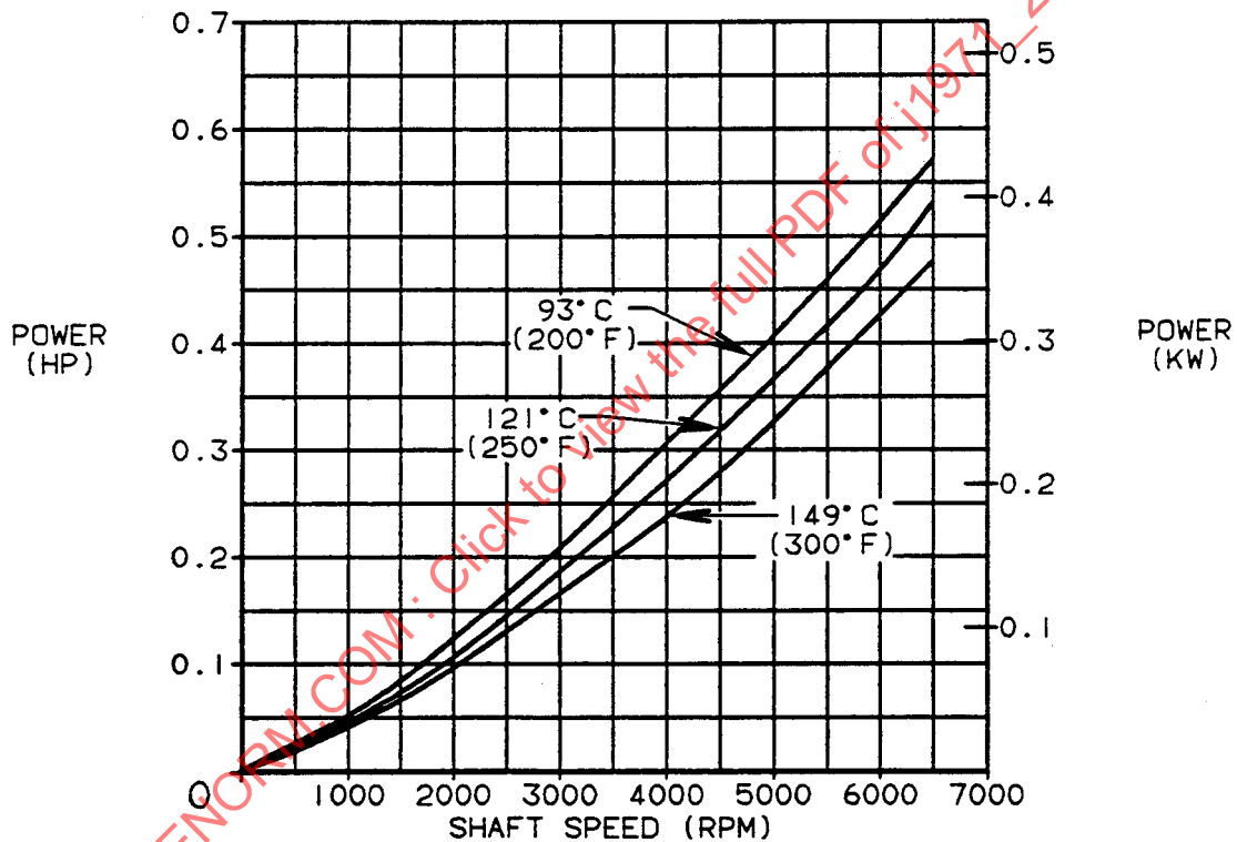
FIGURE 8—EFFECT OF SUMP TEMPERATURE ON SEAL POWER CONSUMPTION
