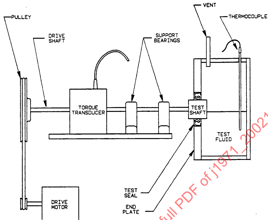
FIGURE 3—ELECTRONIC TORQUE MEASURING MACHINE
