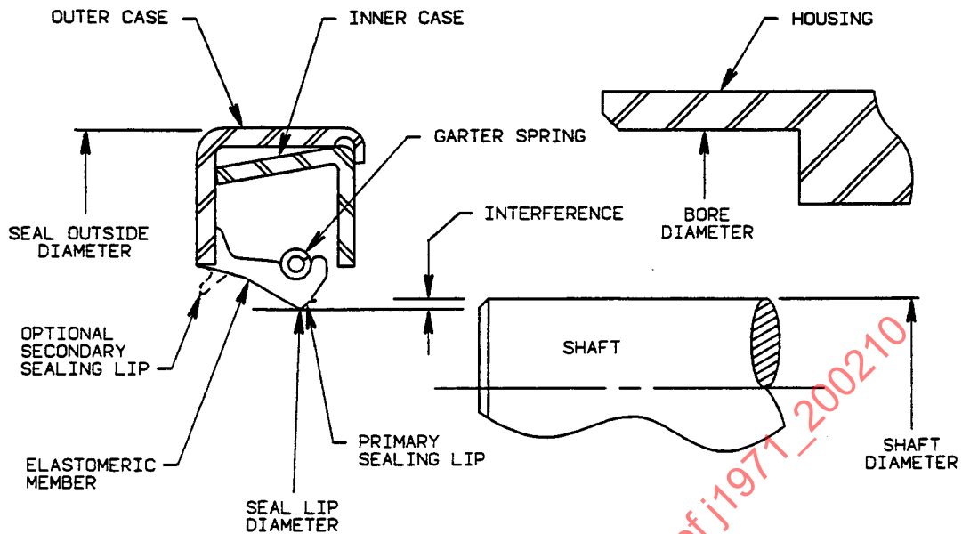
FIGURE 1—TYPICAL RADIAL LIP OIL SEAL
