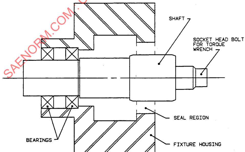
FIGURE 2—FIXTURE TO MEASURE SEAL TORQUE WITH TORQUE WRENCH
