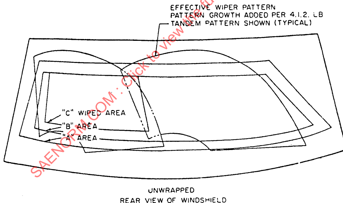
FIGURE 2—WIPED AREA EVALUATION, DRAFTING TEST PROCEDURE—UNWRAPPED VIEW SHOWING WIPED PATTERN AND AREAS A, B, AND C
