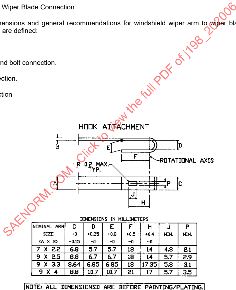
Figure 2 - Hook attachment
