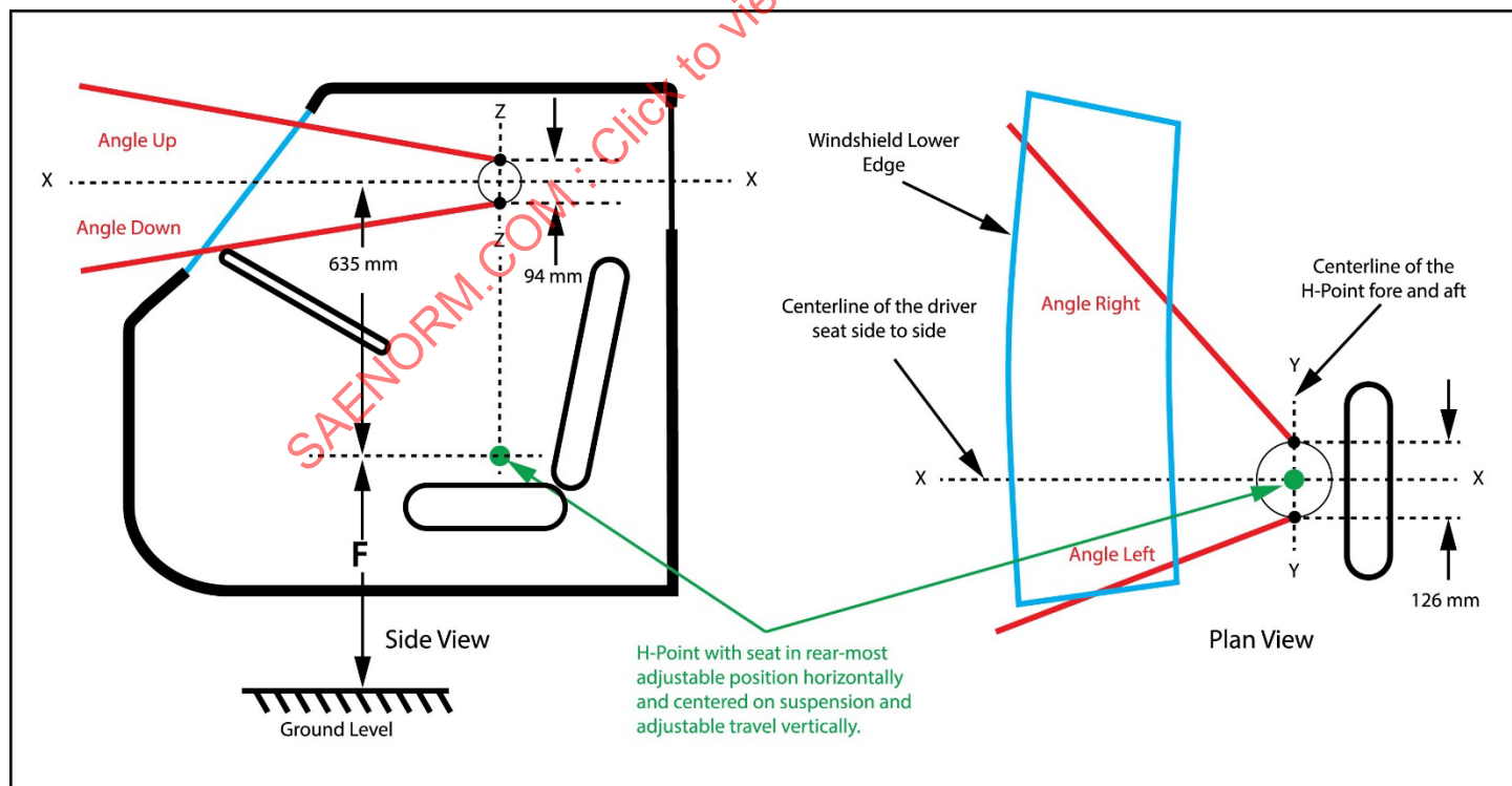
Figure 1 - Target windshield viewing area construction
