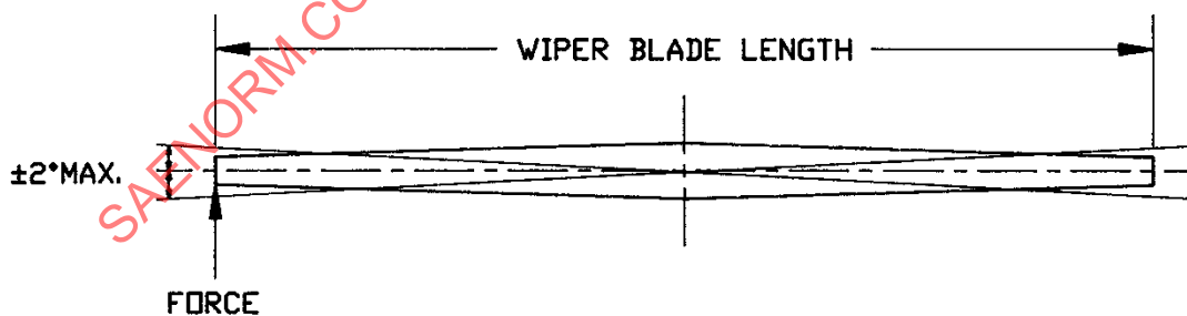
Figure 5 - Lateral angular movement - wiper blade to wiper arm
