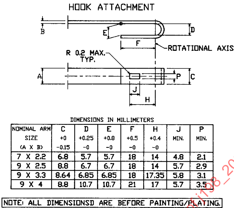
Figure 2 - Hook attachment
