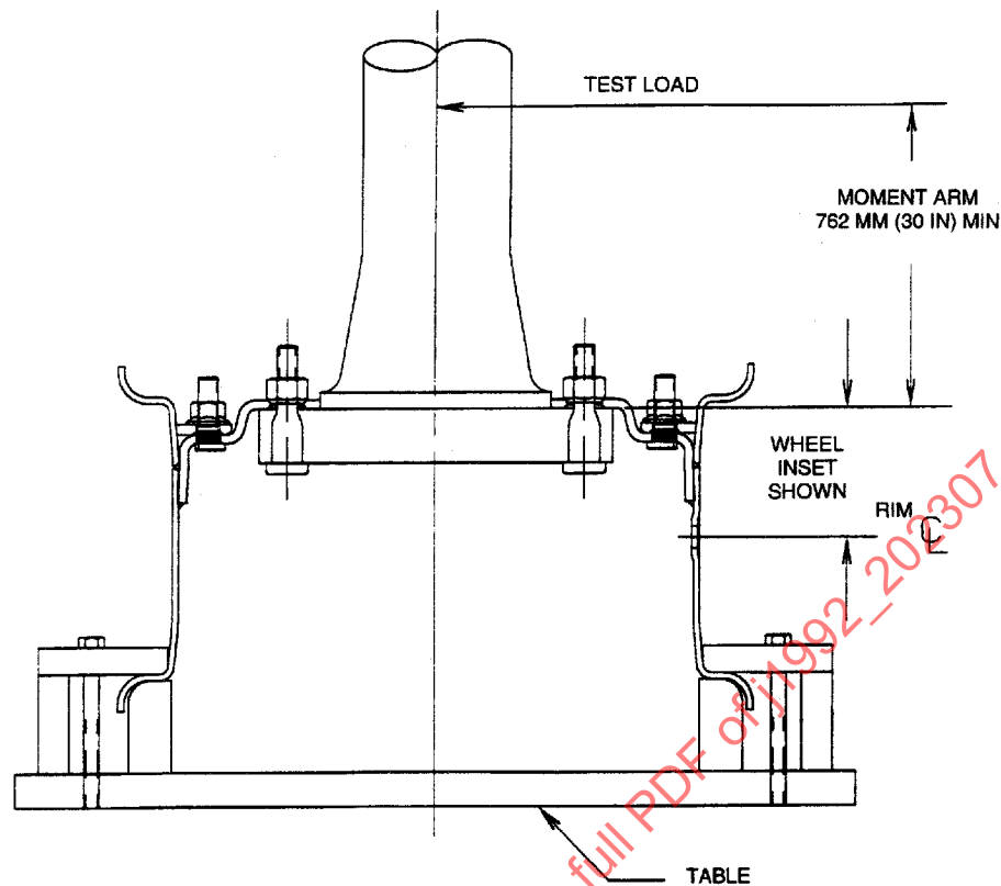
Figure 2B - Cornering fatigue test for bolt-together divided wheels (typical setup)
