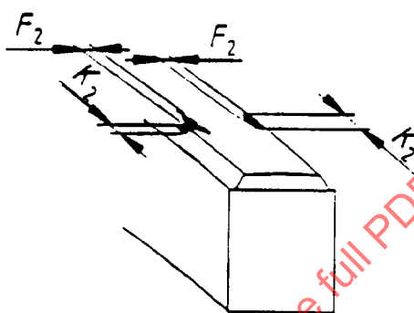
FIGURE 2—CHIPPING ON PERIPHERAL EDGES
