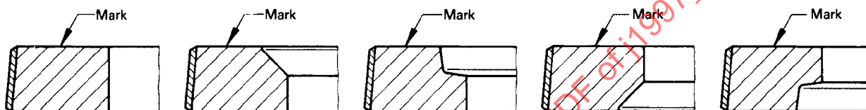
FIGURE 13 – Fully Faced Coated Type M Rings
