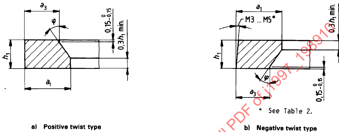
FIGURE 20 - Variable Internal Bevel
