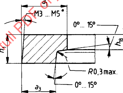
FIGURE 19 – Internal Step Bottom Side (IWU)
