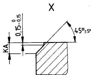
FIGURE 23 – Outside and Inside Chamfered Edges (KA + KI)
