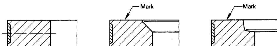
FIGURE 7 – Inlaid Coated Type R Rings
