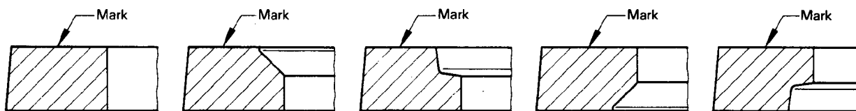
FIGURE 12 – Uncoated Type M Rings
