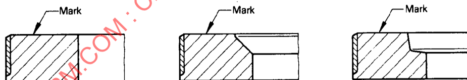
FIGURE 5 – Fully Faced Coated Type R Rings
