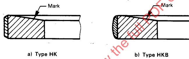
FIGURE 4 – Fully Faced Coated Rings
