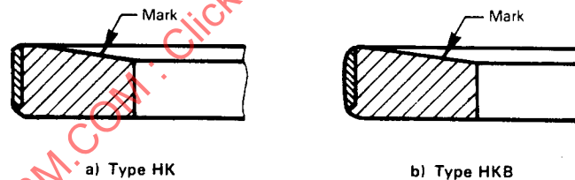
FIGURE 5 – Semi-Inlaid Coated Rings
