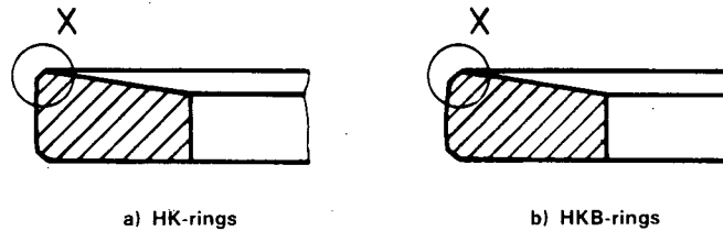
FIGURE 7 – Outside Chamfered Edges (KA)
