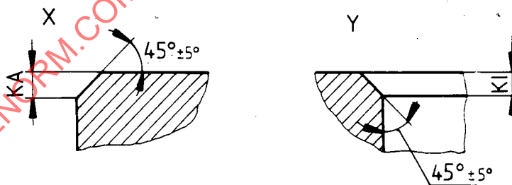
FIGURE 9 – Outside and Inside Chamfered Edges (KA + KI)
