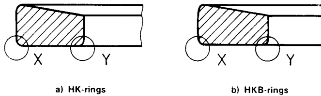
FIGURE 11 - Outside and Inside Rounded Edges
