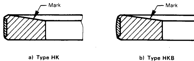
FIGURE 6 – Inlaid Coated Rings
