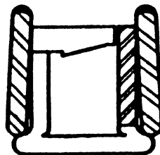
FIGURE 4—ES-3 TYPE
