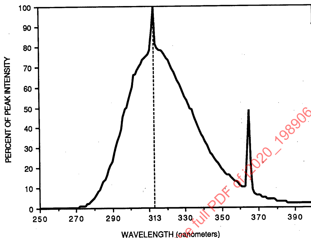
FIGURE 1 - Typical Relative SPD of FS-40 (F40 UVB) Lamp
