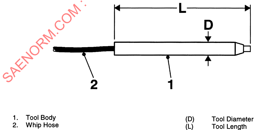
FIGURE 5—PIERCING TOOL
