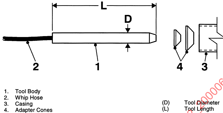
FIGURE 6—RAMMING MACHINE
