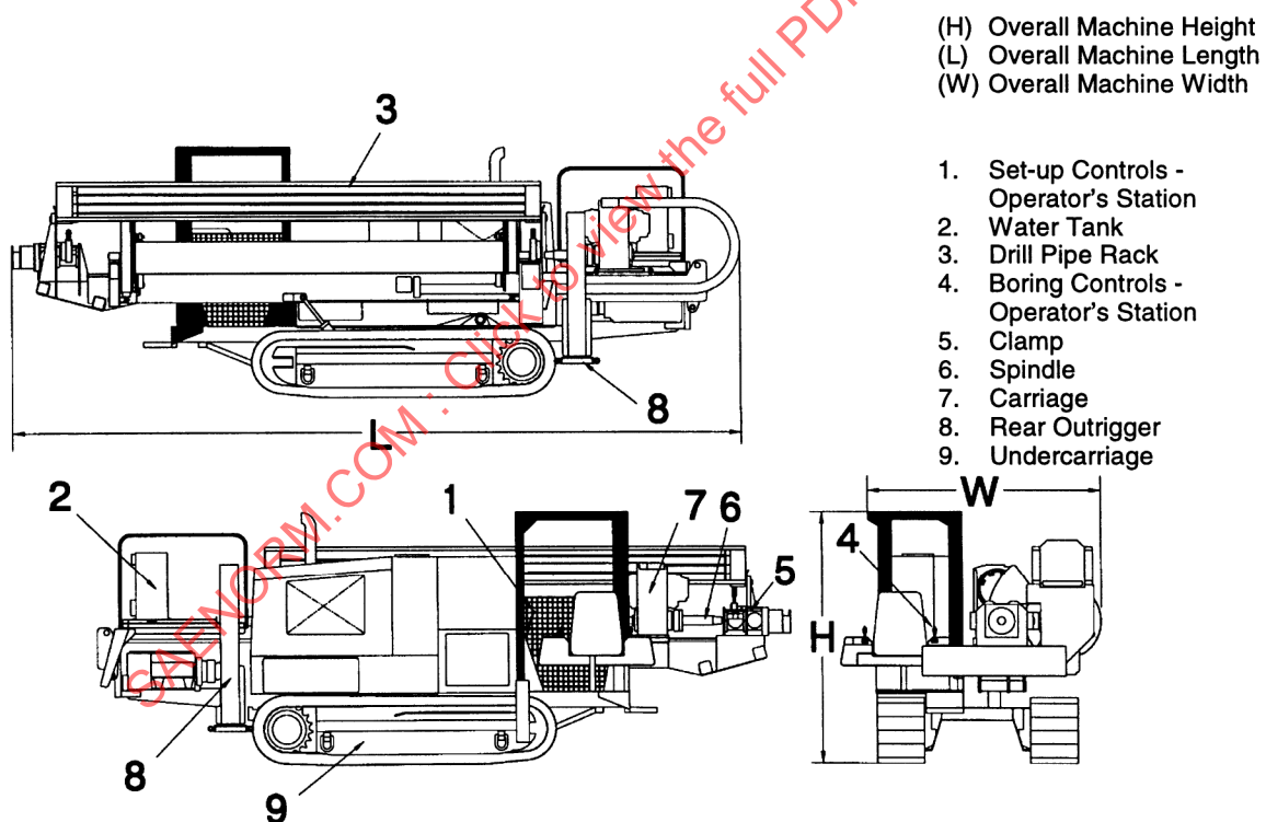
FIGURE 8—DIRECTIONAL BORING/DRILLING MACHINES—RIDE-ON UNITS
