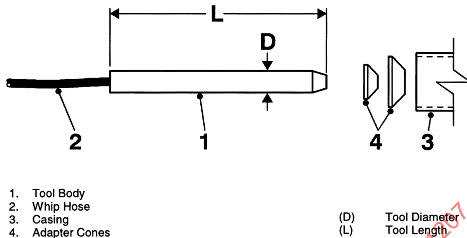
FIGURE 6—RAMMING MACHINE
