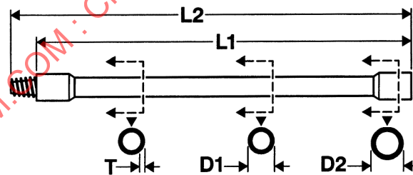
FIGURE 11—DRILL PIPE
