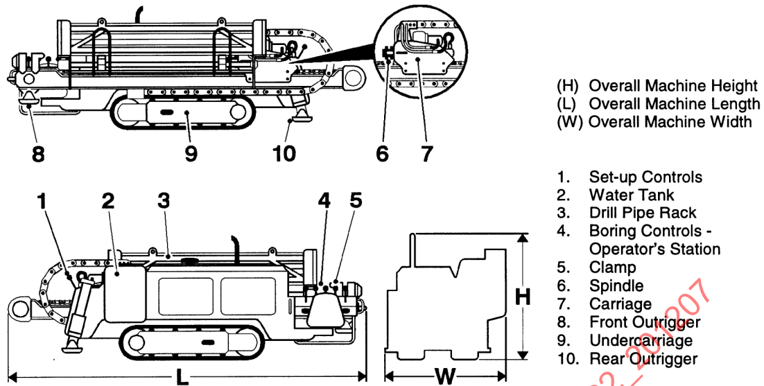
FIGURE 7—DIRECTIONAL BORING/DRILLING MACHINES—WALK-ALONG UNITS
