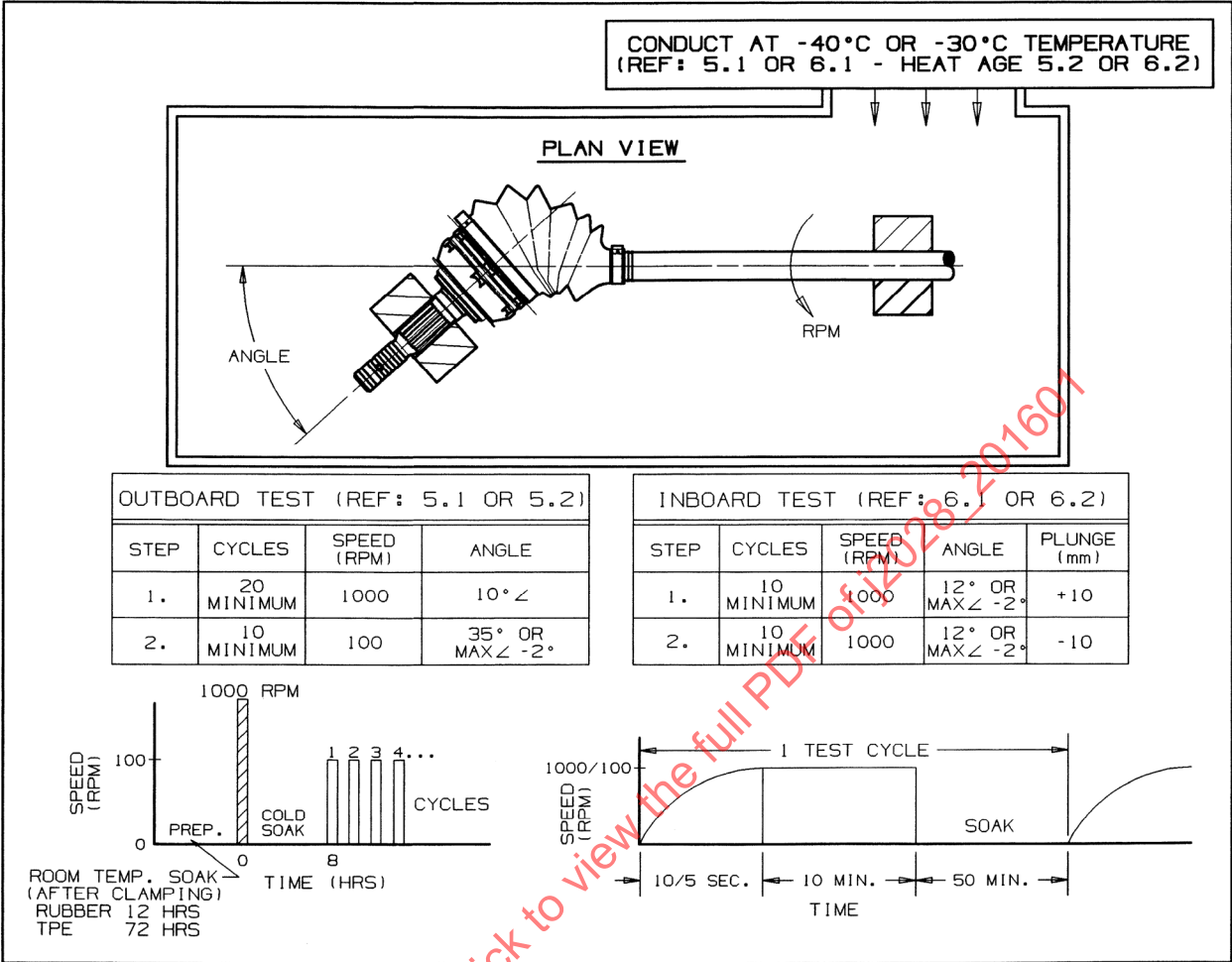
FIGURE 1—COLD TEST
