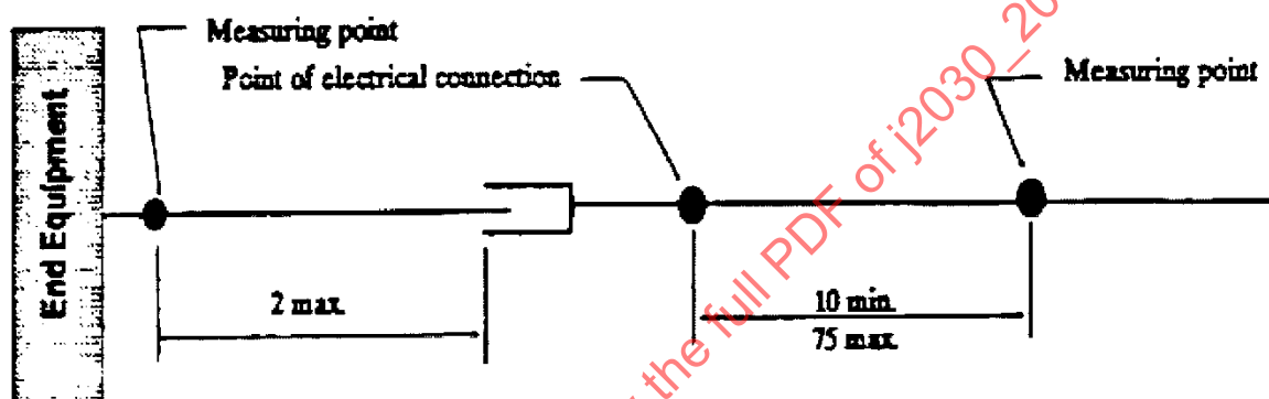
FIGURE 1 - CONNECTION RESISTANCE, CABLE TO CABLE
