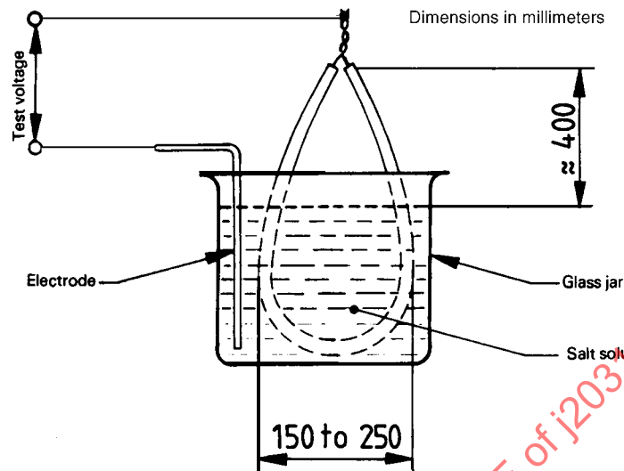
FIGURE A1 - TEST APPARATUS FOR HIGH POTENTIAL TEST
