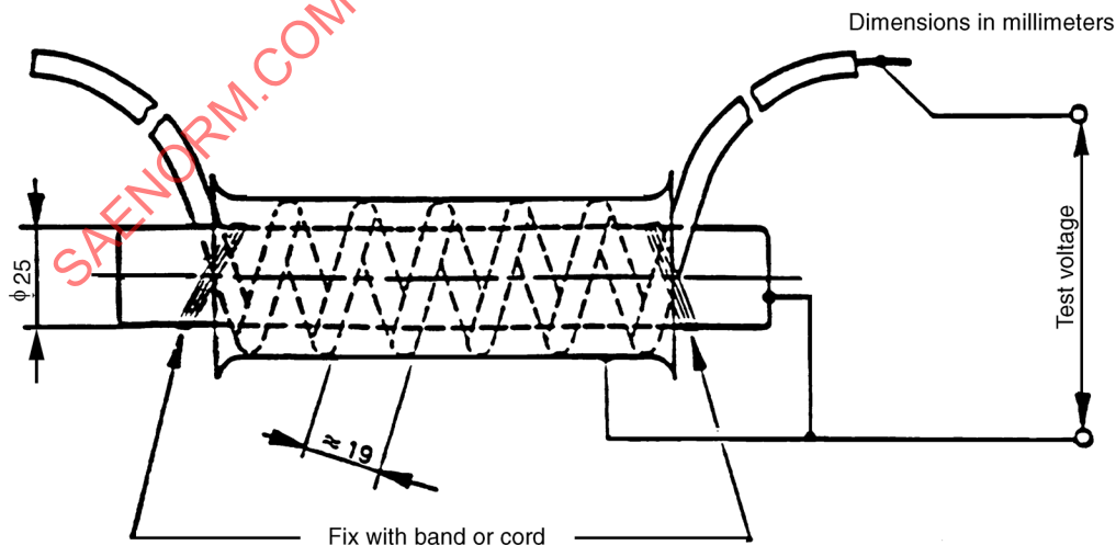
Figure A2 - Test apparatus for corona resistance test
