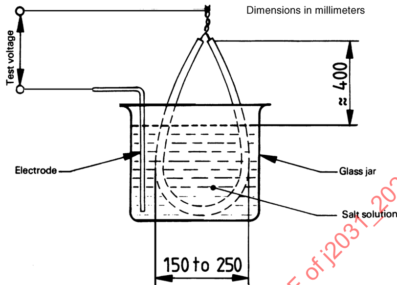
Figure A1 - Test apparatus for high potential test
