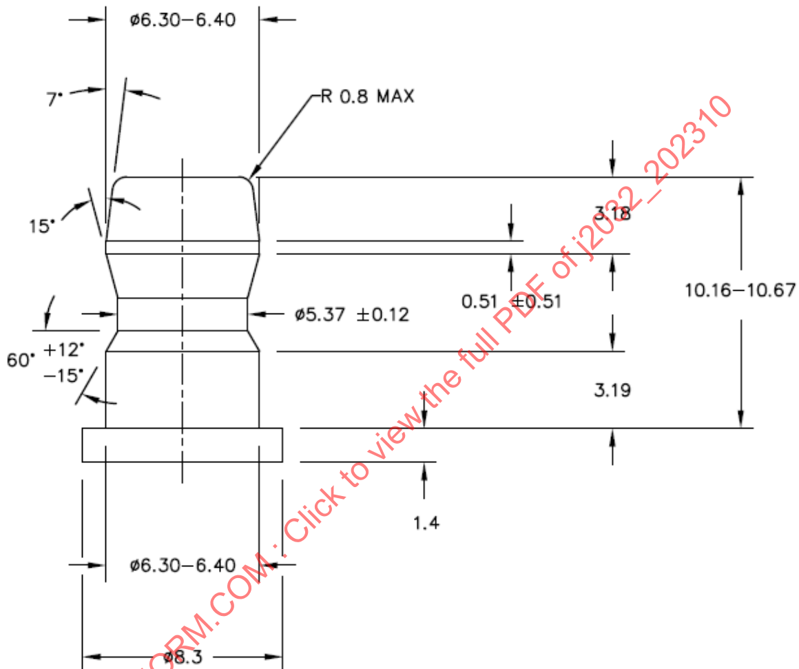
Figure 1 - Gage for measurement of insertion and removal forces of high-voltage connectors for spark plugs with post type terminals and for ignition coil and distributors with plug type high-voltage connections
