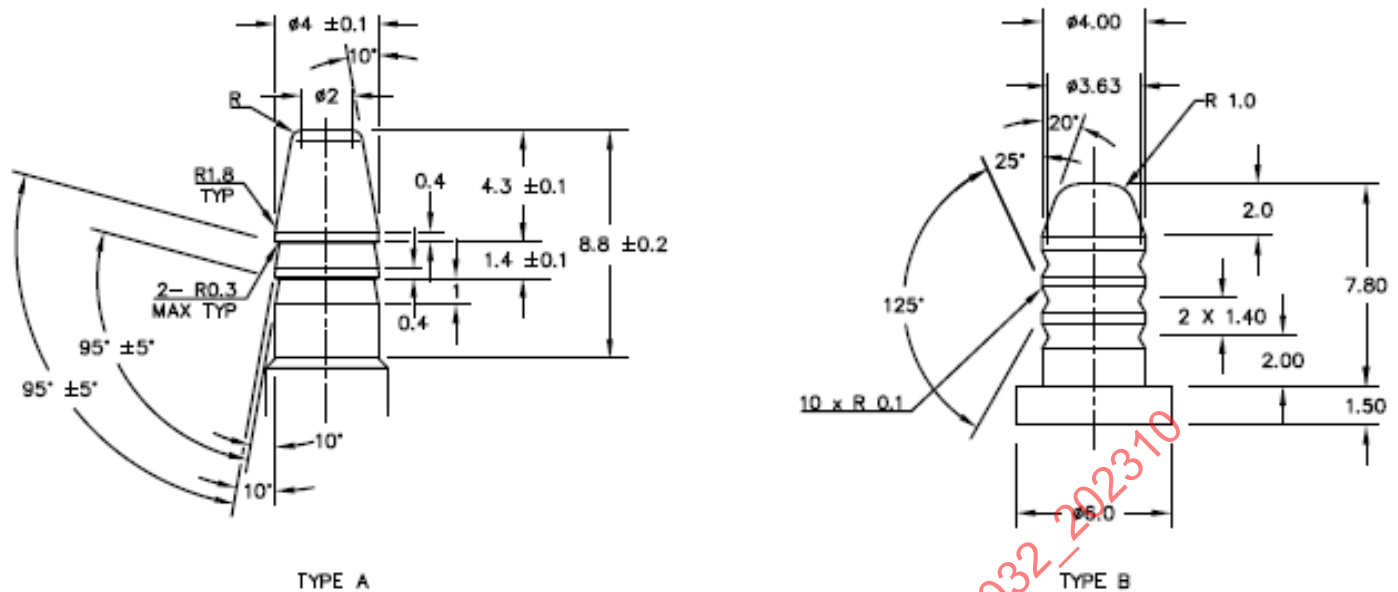
Figure 4 - Gage for measurement of insertion and removal forces of high-voltage connectors for 4 mm stud high-voltage connection for ignition coils and distributors
