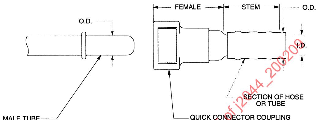
FIGURE 1—CONNECTOR NOMENCLATURE
