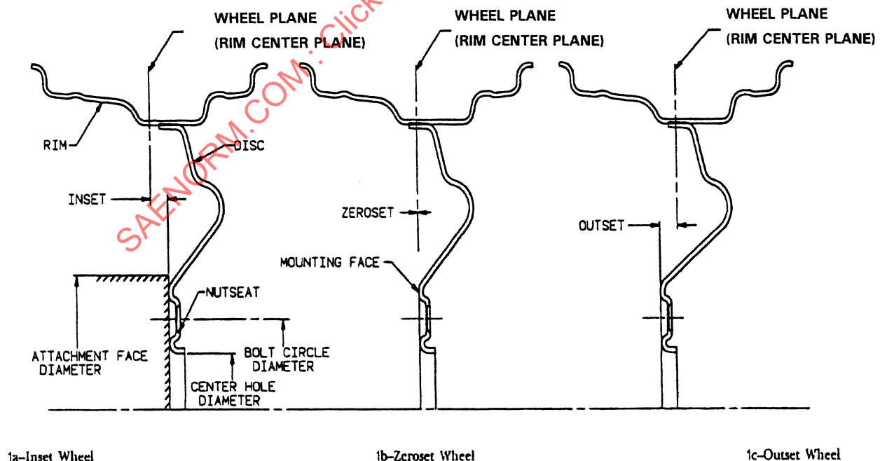
FIGURE 1—WHEEL OFFSET
