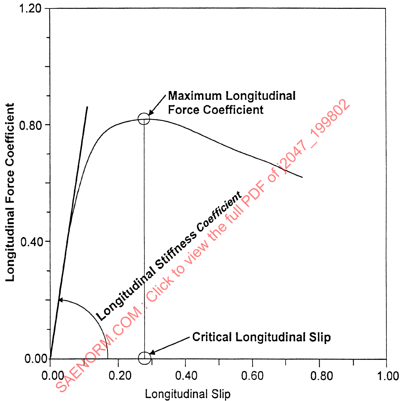
FIGURE 16—EXAMPLE OF LONGITUDINAL FORCE COEFFICIENT VERSUS LONGITUDINAL SLIP
