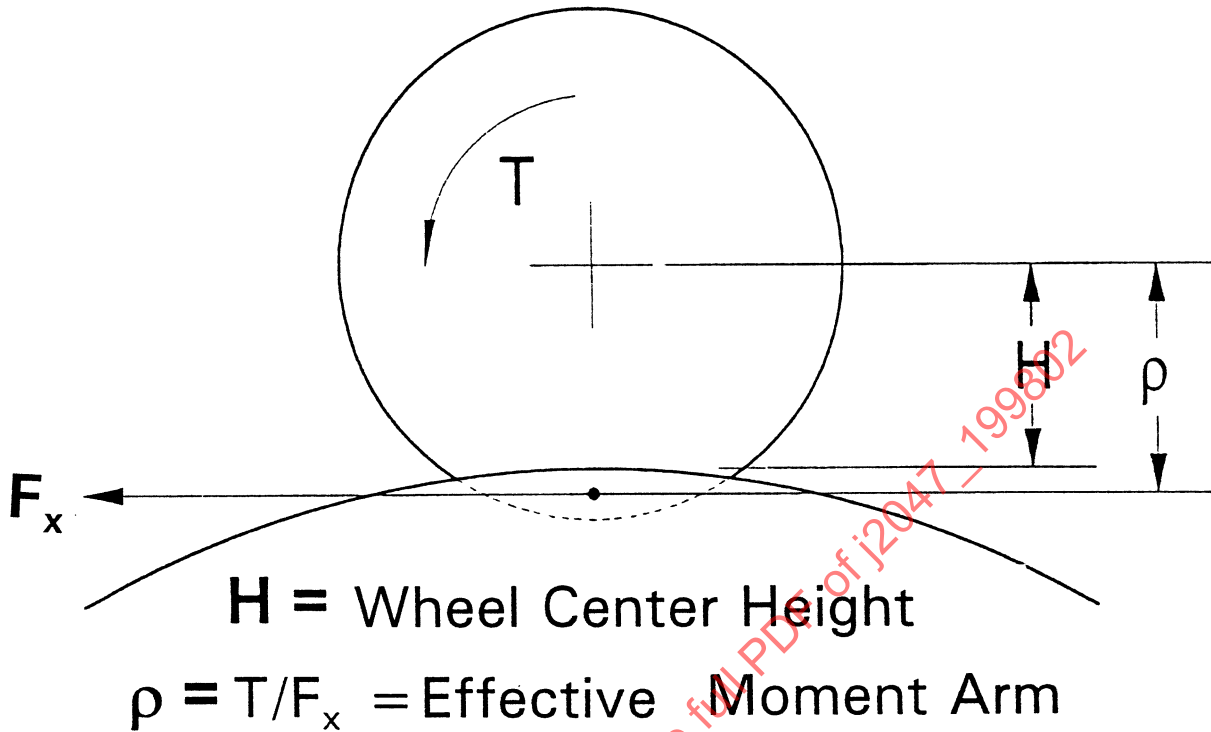
FIGURE 5—WHEEL CENTER HEIGHT AND EFFECTIVE MOMENT ARM FOR A CURVED ROAD SURFACE
