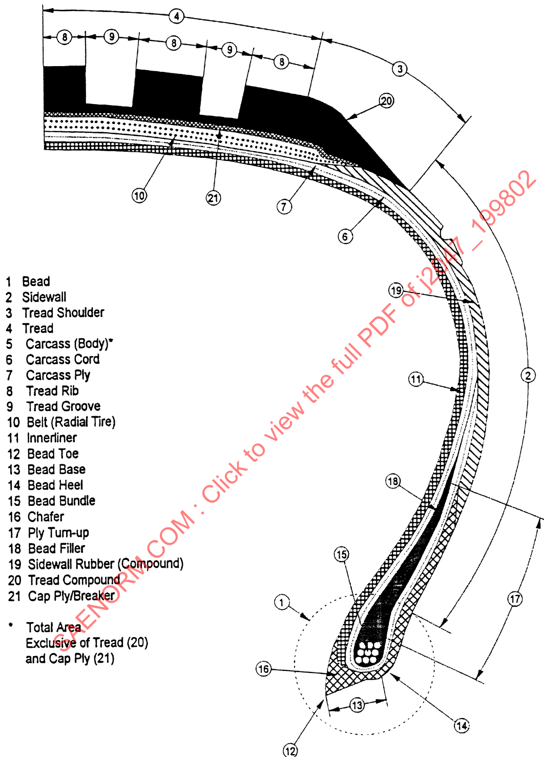
FIGURE 4—TIRE COMPONENTS AND TIRE ELEMENTS
