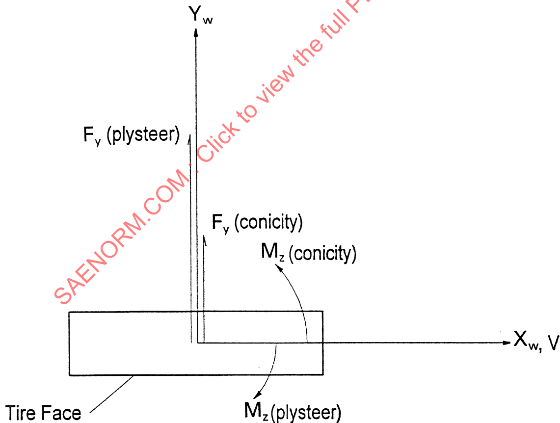
FIGURE 14—PLYSTEER AND CONICITY FORCES DURING CLOCKWISE WHEEL ROTATION
