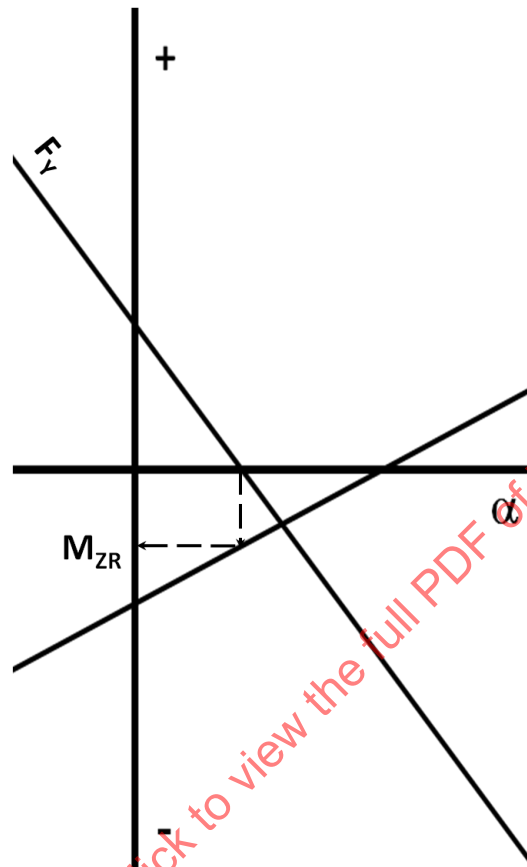
FIGURE 16 – RESIDUAL ALIGNING MOMENT
