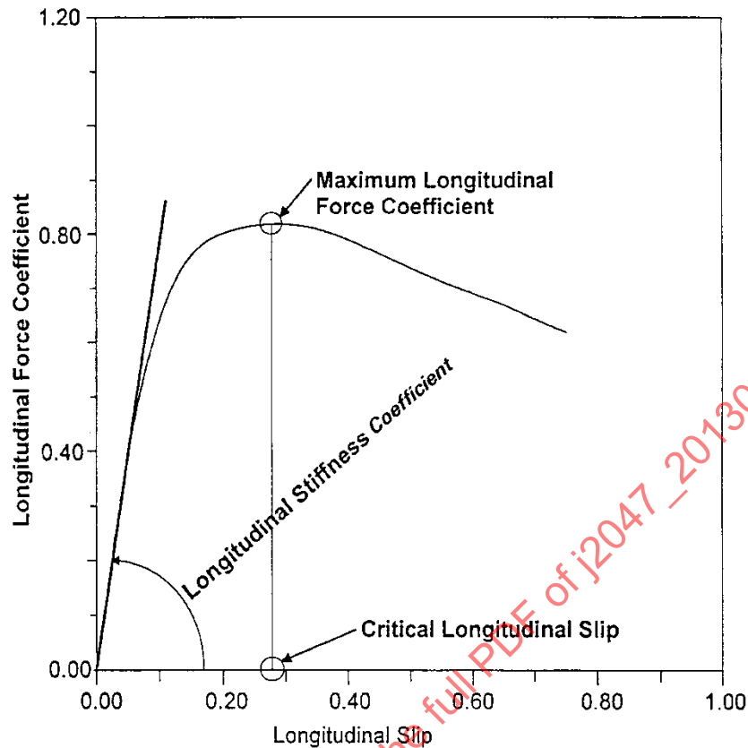
FIGURE 17 - EXAMPLE OF LONGITUDINAL FORCE COEFFICIENT VERSUS LONGITUDINAL SLIP
