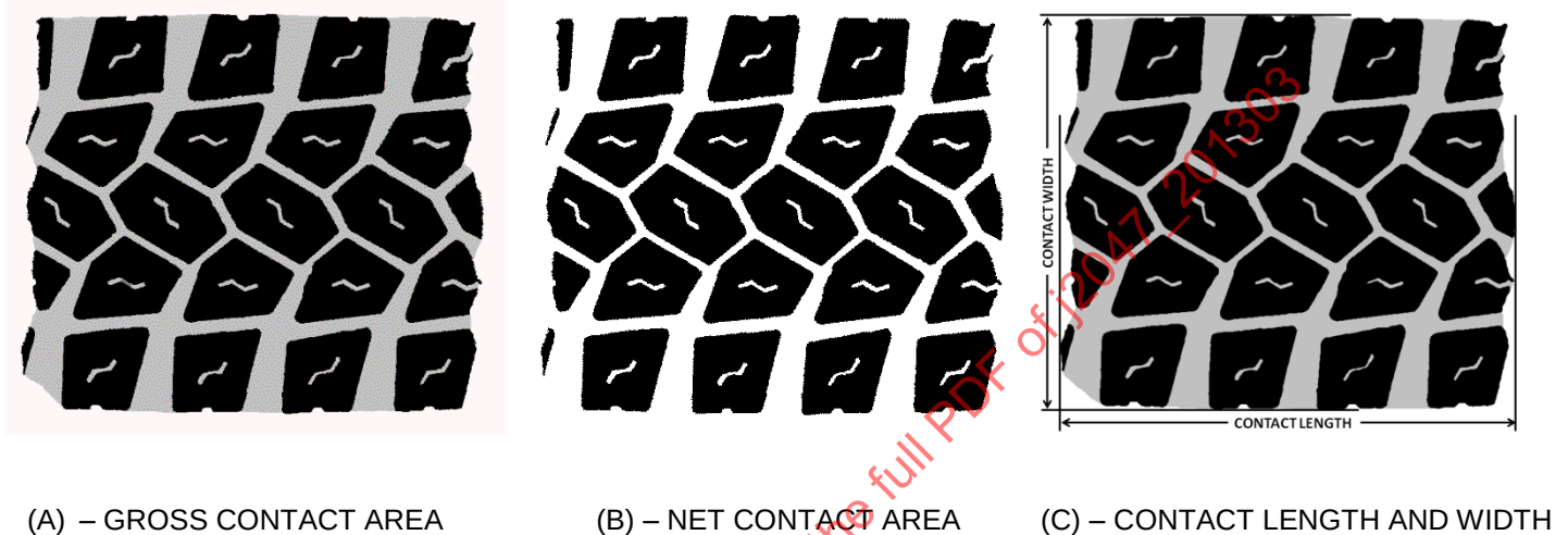
FIGURE 6 – CONTACT AREAS AND DIMENSIONS
