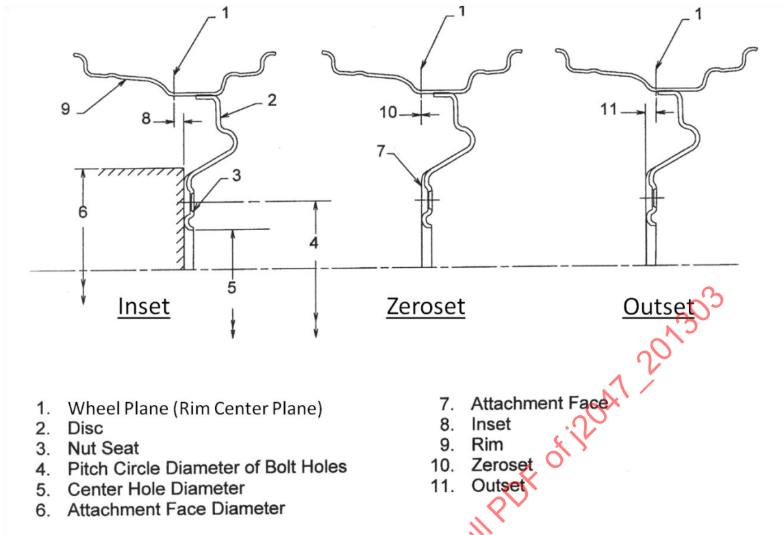
FIGURE 1 - WHEEL OFFSET (RIM TO DISC OFFSET - SAE J1982)
