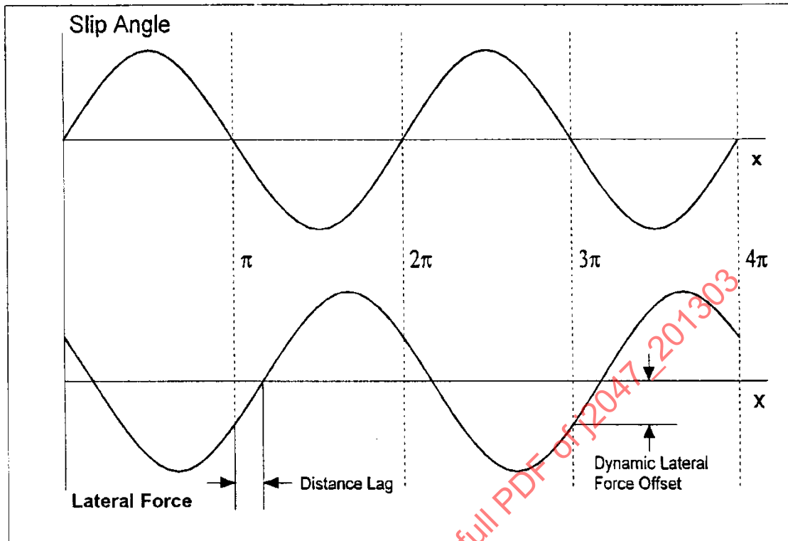
FIGURE 20 - LATERAL FORCE RESPONSE TO A SINUSOIDAL SLIP ANGLE INPUT
