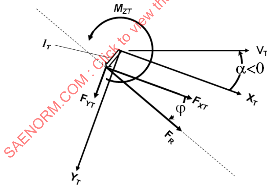
FIGURE 11A – TIRE FORCES AND MOMENTS IN THE ROAD PLANE – Z – UP
