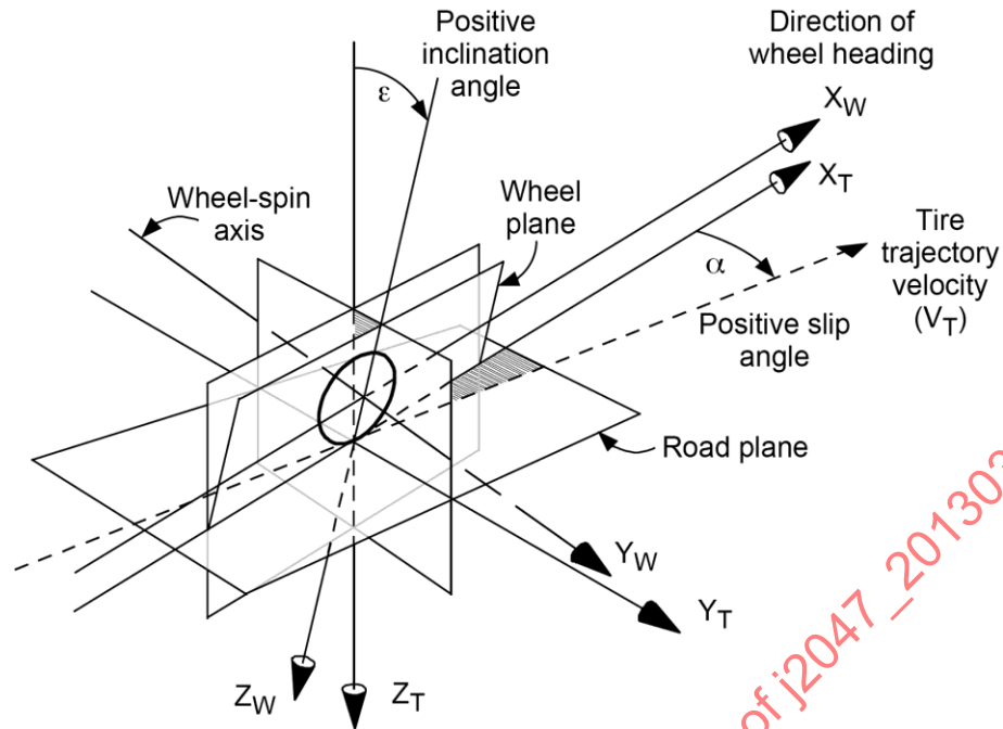
FIGURE 9B - TIRE AND WHEEL AXIS SYSTEM – Z-DOWN
