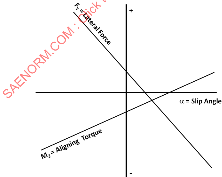
FIGURE 14 – LATERAL FORCE AND ALIGNING TORQUE FOR A TYPICAL TIRE NEAR ZERO SLIP ANGLE
