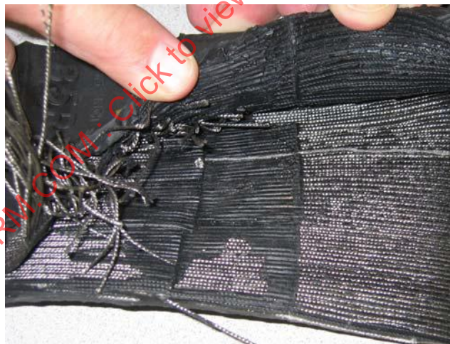
FIGURE 28 - CORD SEPARATION
