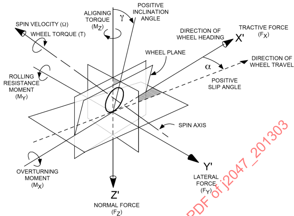
FIGURE 10C – FORCE AND MOMENT NOMENCLATURE – HISTORIC SAE
