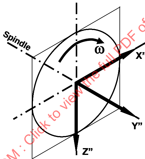
FIGURE 9D – SAE PARALLEL TIRE COORDINATE SYSTEM
