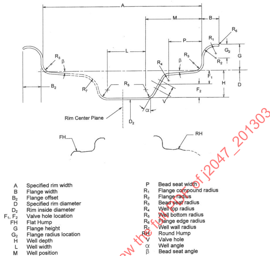
FIGURE 2 – RIM (SAE J1982)
