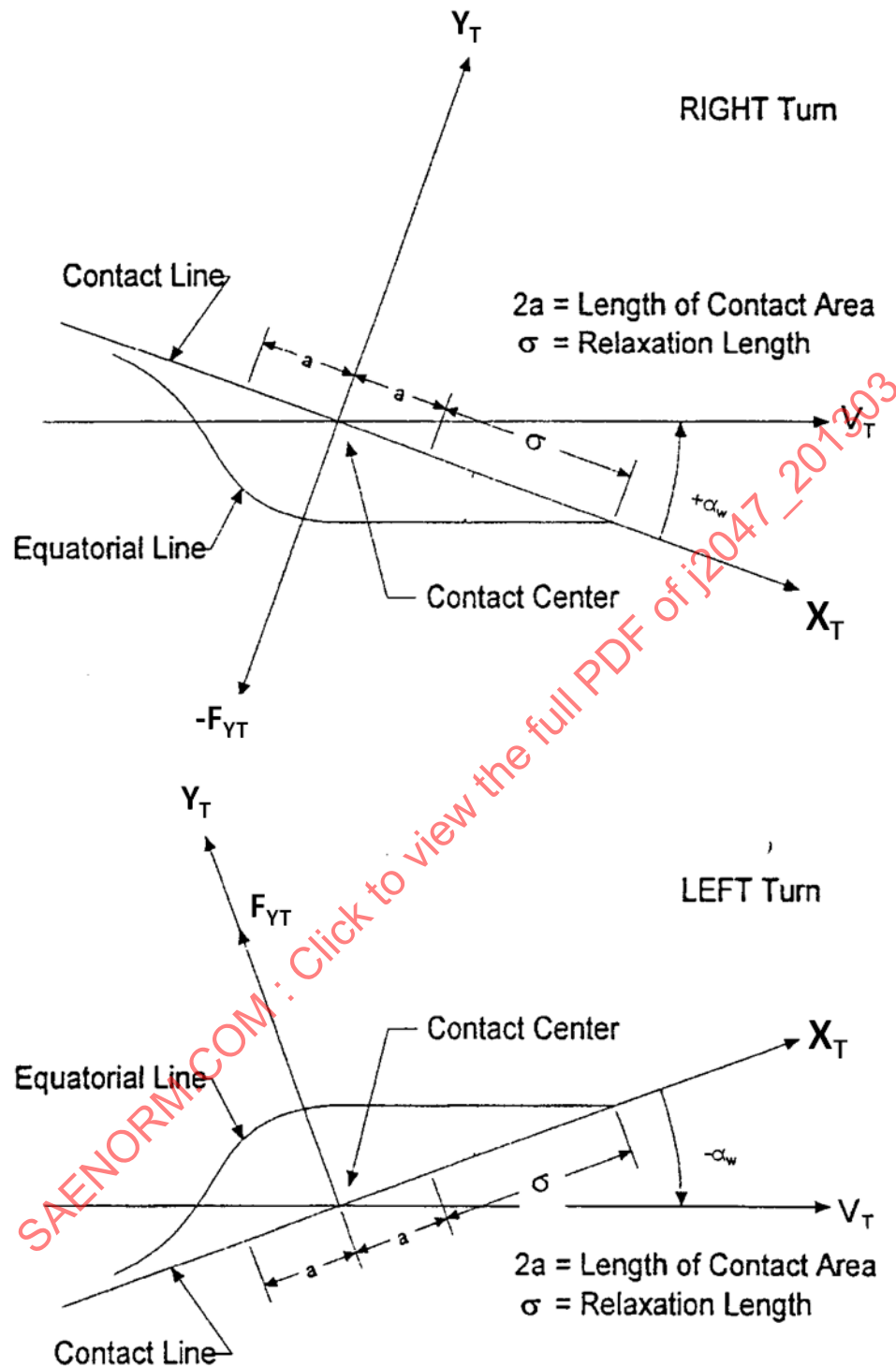
FIGURE 19 - DEFORMED EQUATORIAL LINE OF A TIRE TURNING LEFT AND RIGHT Z-UP AXIS SYSTEM USED.
