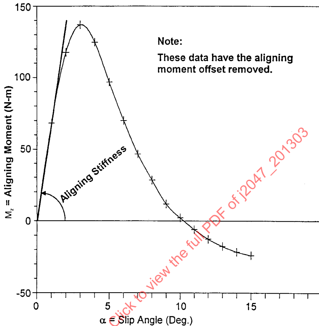
FIGURE 23 - EXAMPLE OF ALIGNING MOMENT VERSUS SLIP ANGLE
