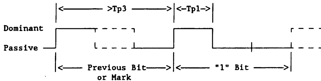
"1" Bit Definition
