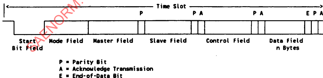
FIGURE 18—SIX FIELD MESSAGE FORMAT
