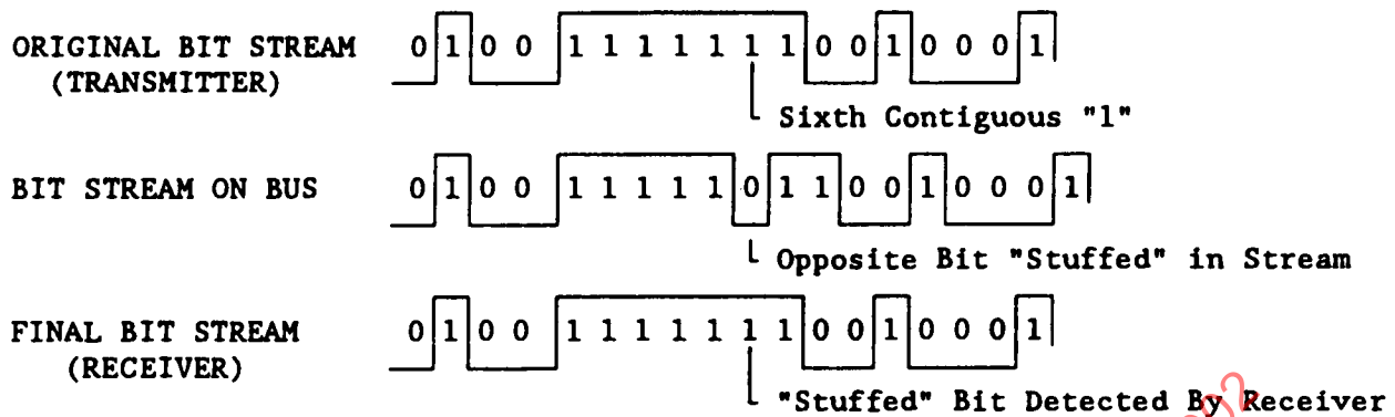
FIGURE 11—NRZ BIT "STUFFING"
