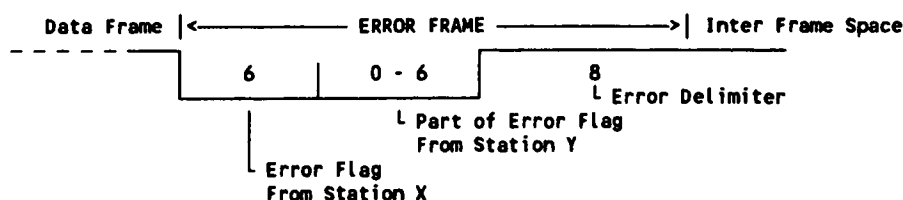
FIGURE 14—ERROR FRAME
