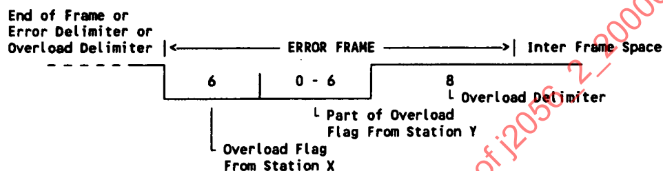
FIGURE 15—OVERLOAD FRAME
