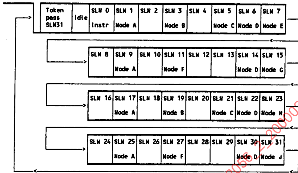
FIGURE 29—A TYPICAL TOKEN SLOT NODE ASSIGNMENT AND SLOT SEQUENCE CYCLE PATTERN
