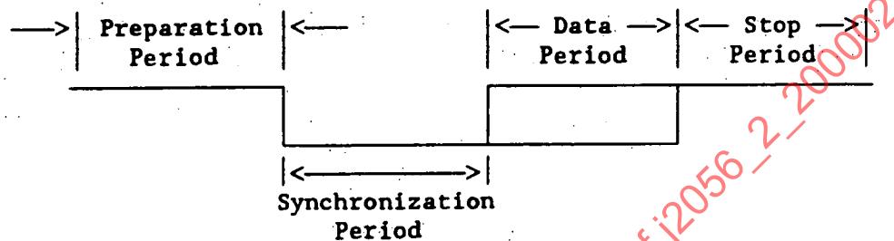
FIGURE 17—PULSE WIDTH MODULATION BIT FORMAT
