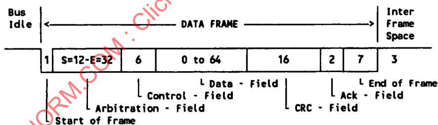
FIGURE 12—DATA FRAME
