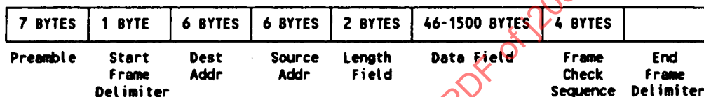
FIGURE 19—SEVEN FIELD MESSAGE FORMAT
