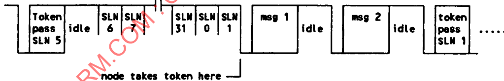
FIGURE 31—TYPICAL TOKEN PASS SEQUENCE
