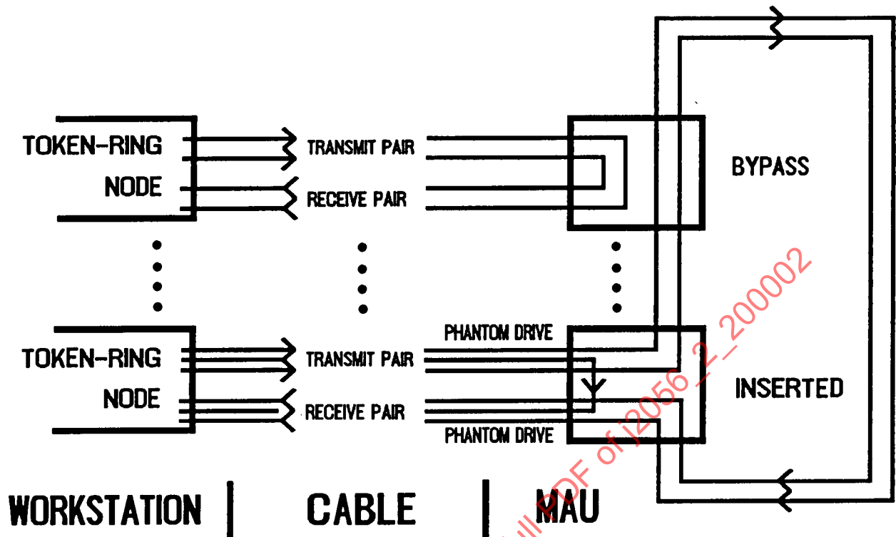
FIGURE 25—TOKEN RING PHYSICAL INTERFACE
