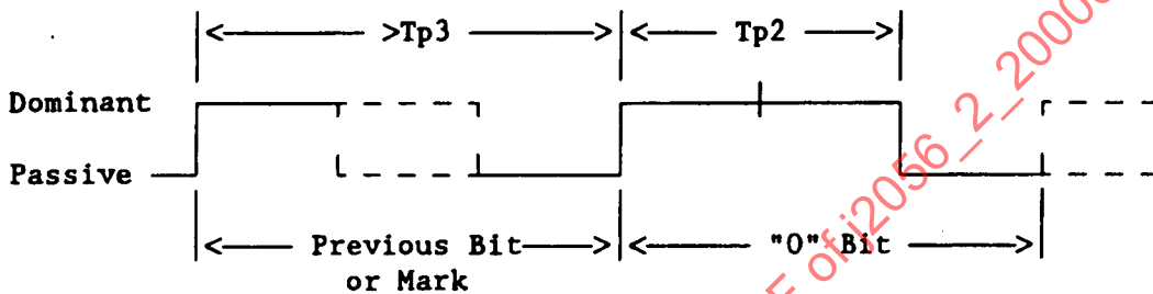
"0" Bit Definition
