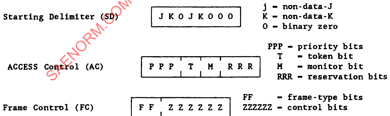
FIGURE 28—FRAME CONFIGURATION
