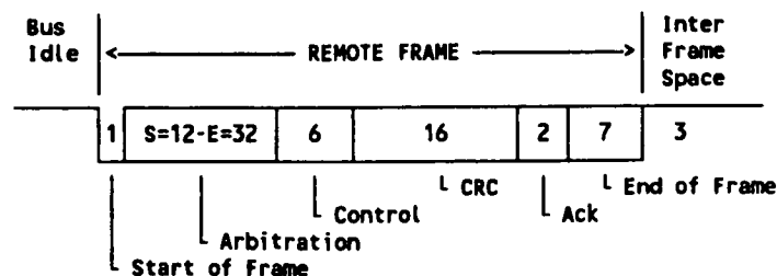
FIGURE 13—REMOTE FRAME
