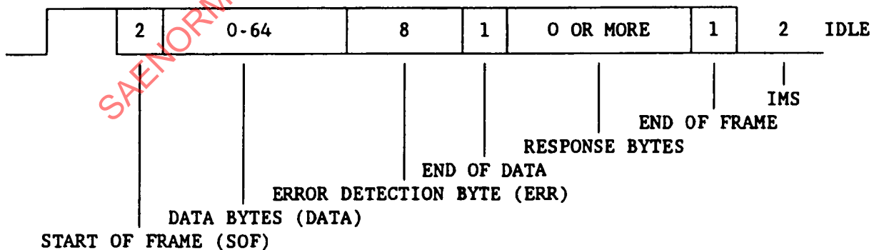
FIGURE 10—SAE J1850 MESSAGE FRAME
