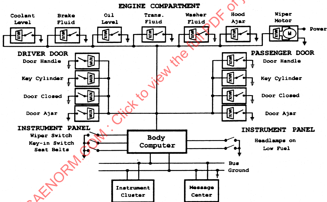
FIGURE 8—DATA LINK WITH BODY COMPUTER, INSTRUMENT CLUSTER, MESSAGE CENTER, AND CLASS A NETWORK FOR SENSORS
