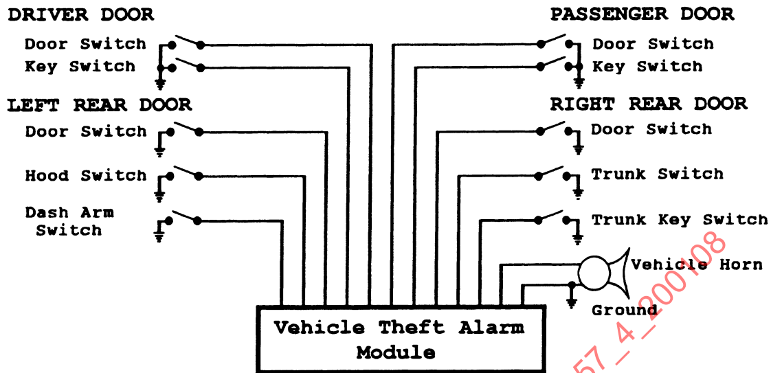
FIGURE 2—EXAMPLE VEHICLE THEFT ALARM SYSTEM
