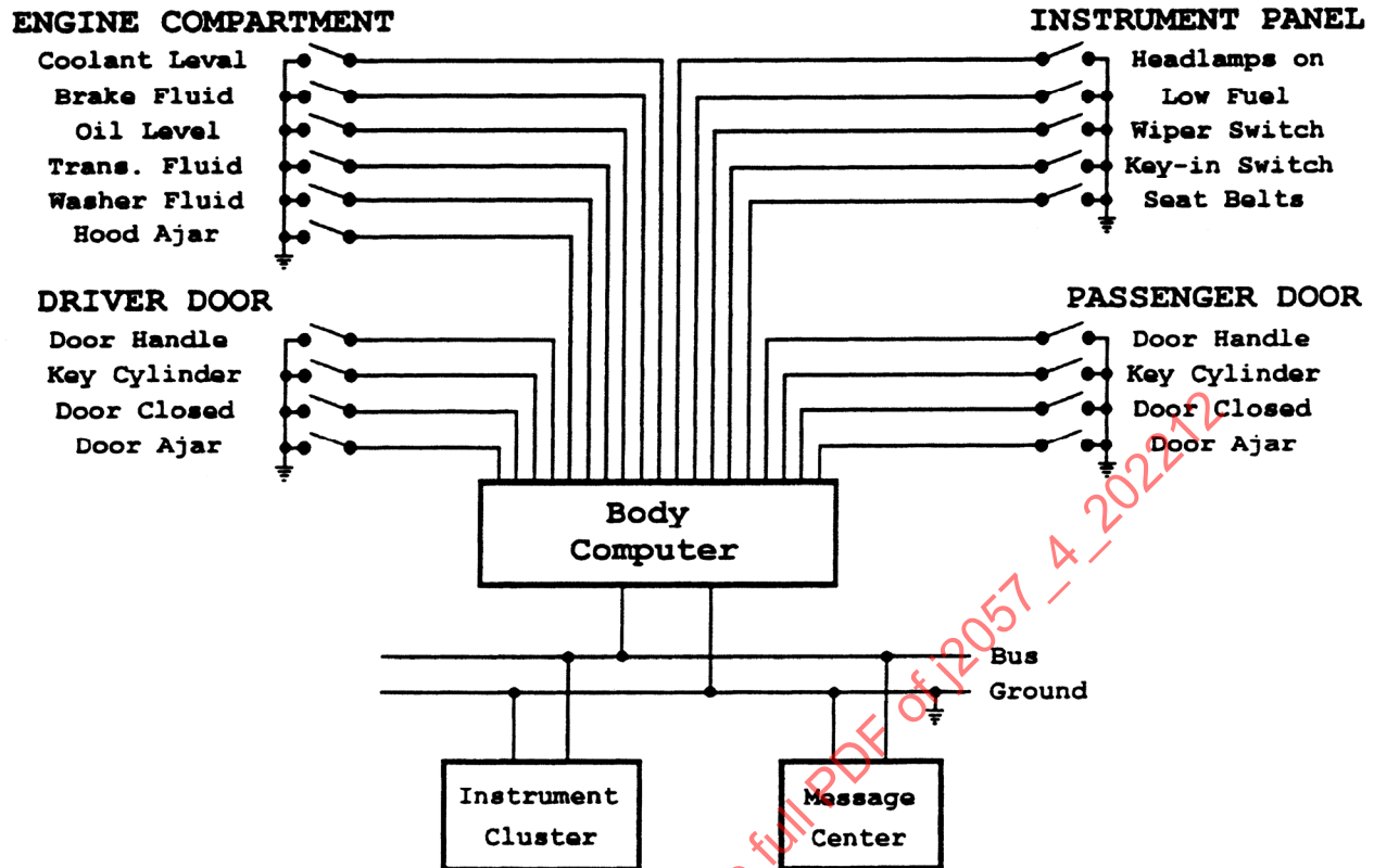
FIGURE 4 - DATA COMMUNICATIONS NETWORK WITH BODY COMPUTER, INSTRUMENT CLUSTER, AND MESSAGE CENTER
