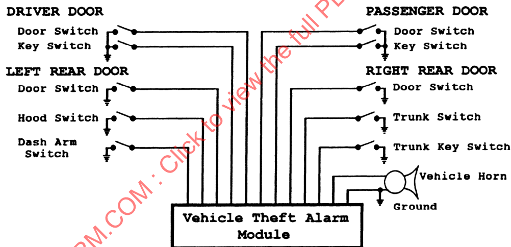
FIGURE 2 - EXAMPLE VEHICLE THEFT ALARM SYSTEM
