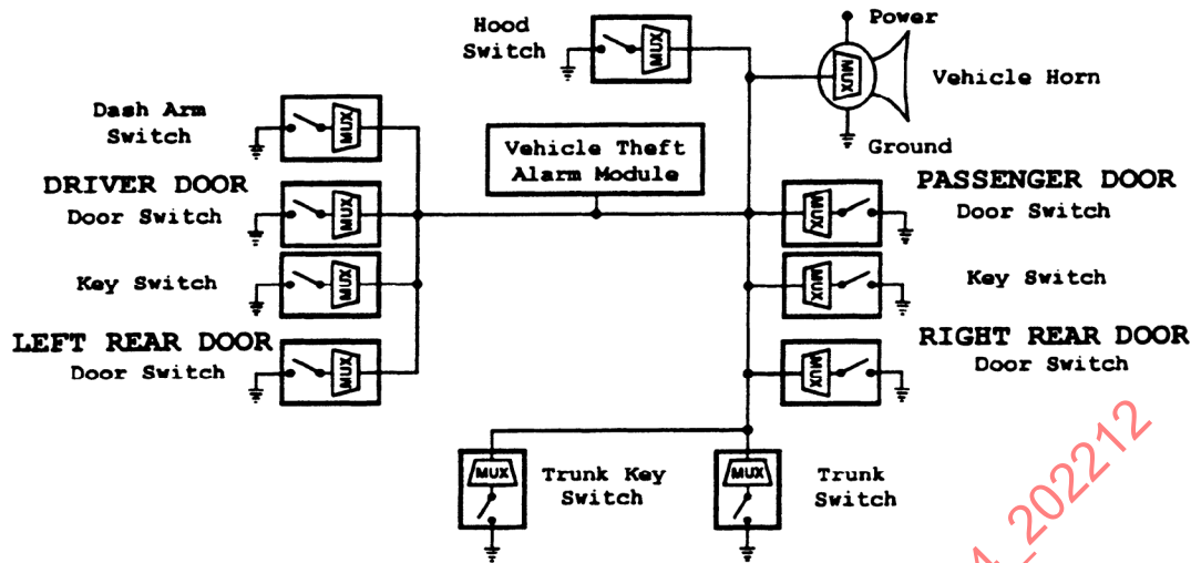
FIGURE 3 - MULTIPLEXED THEFT ALARM SYSTEM
