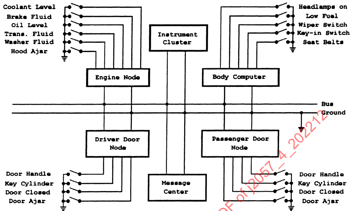
FIGURE 5 - DATA LINK WITH BODY COMPUTER, INSTRUMENT CLUSTER, MESSAGE CENTER AND THREE SENSOR NOTES
