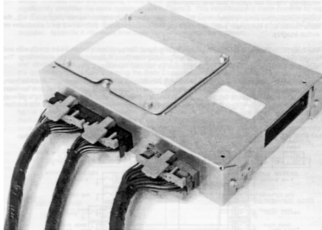
FIGURE 6 - ENGINE CONTROLLER CONNECTOR AND WIRE BUNDLE
