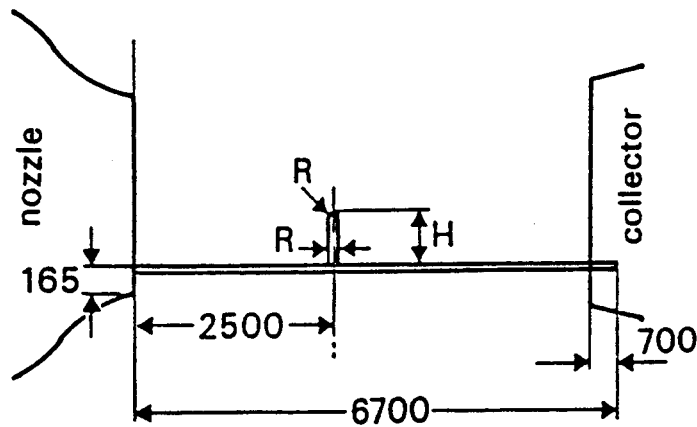
FIGURE 24—TEST ARRANGEMENT AT DLR
