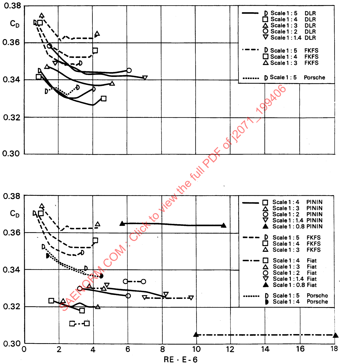
FIGURE 37—DRAG COEFFICIENTS OF MIRA STATION WAGON MODELS
