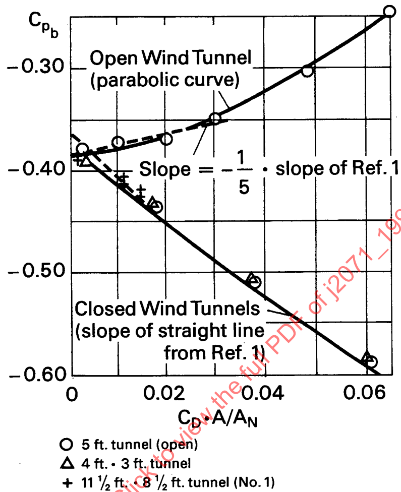
FIGURE 8—BLOCKAGE EFFECT ON BASE PRESSURE. NONLIFTING SQUARE PLATES AFTER REFERENCE 2.1.2 (11)
