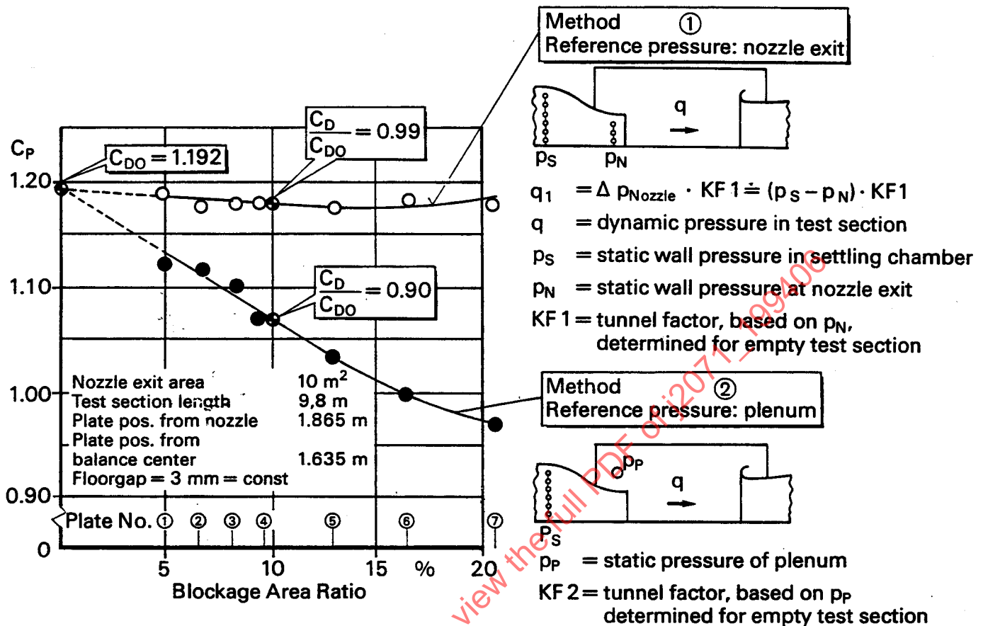
FIGURE 21—DRAG COEFFICIENT OF FLAT PLATES VERSUS BLOCKAGE AREA RATIO A/A_N FOR DIFFERENT METHODS OF DYNAMIC PRESSURE DETERMINATION; MEASUREMENTS FROM BMW ACOUSTIC WIND TUNNEL
