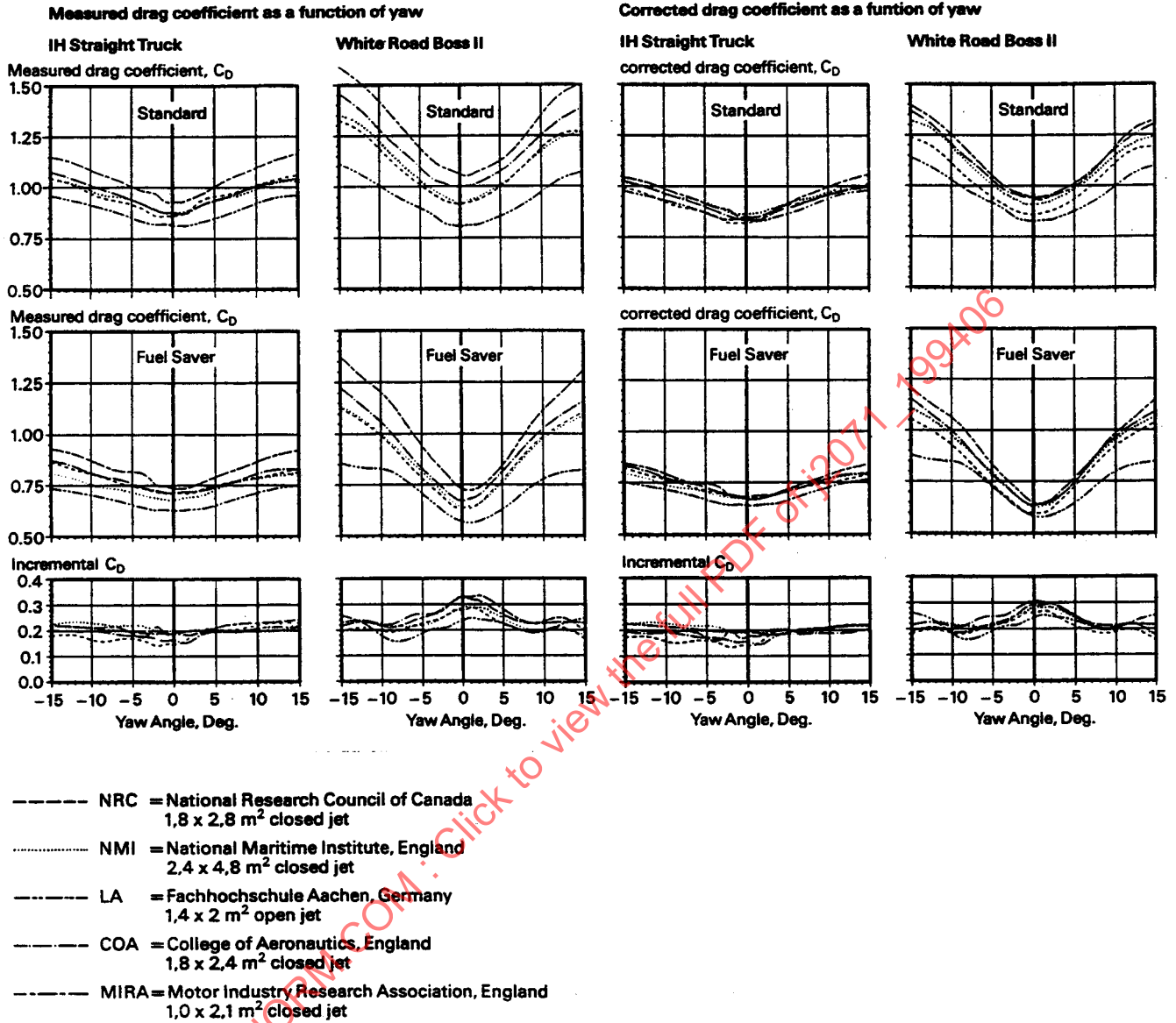
FIGURE 13—DRAG COEFFICIENTS OF 1:10 SCALE TRUCK MODELS IN DIFFERENT WIND TUNNELS AFTER REFERENCE 2.1.2 (15)
