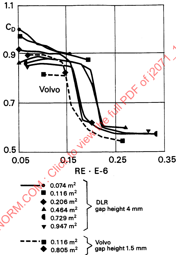
FIGURE 26—DRAG COEFFICIENTS OF PLATE MODELS WITH ROUNDED EDGES FACING THE FLOW
