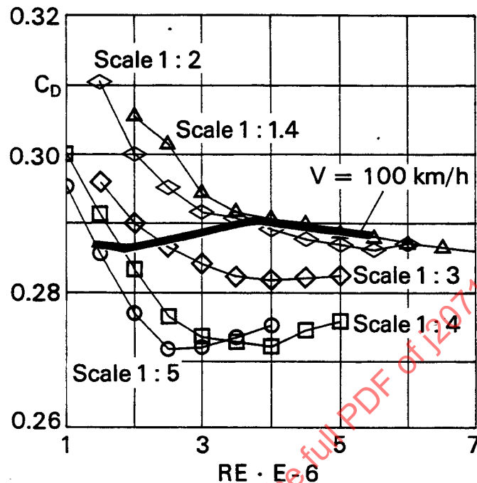
FIGURE 38—DRAG COEFFICIENTS OF MIRA NOTCHBACK MODELS IN DLR WIND TUNNEL
