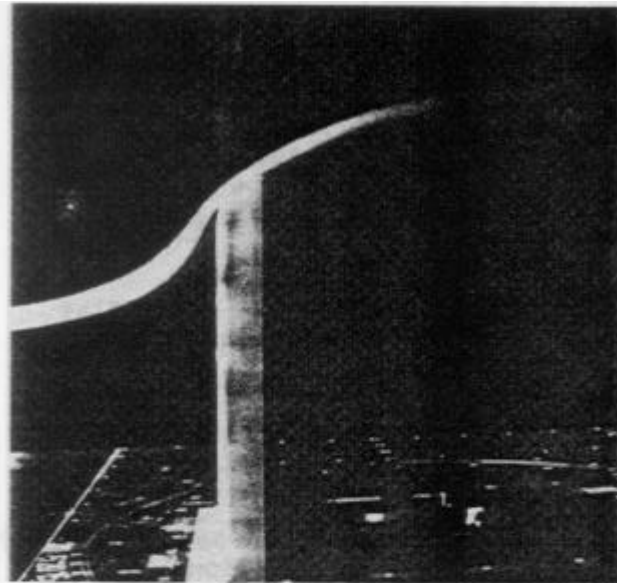
Photo 1 Square flat plate in VOLVO semi open test section Low Reynolds number, separation on the round edge Note the supporting struture
