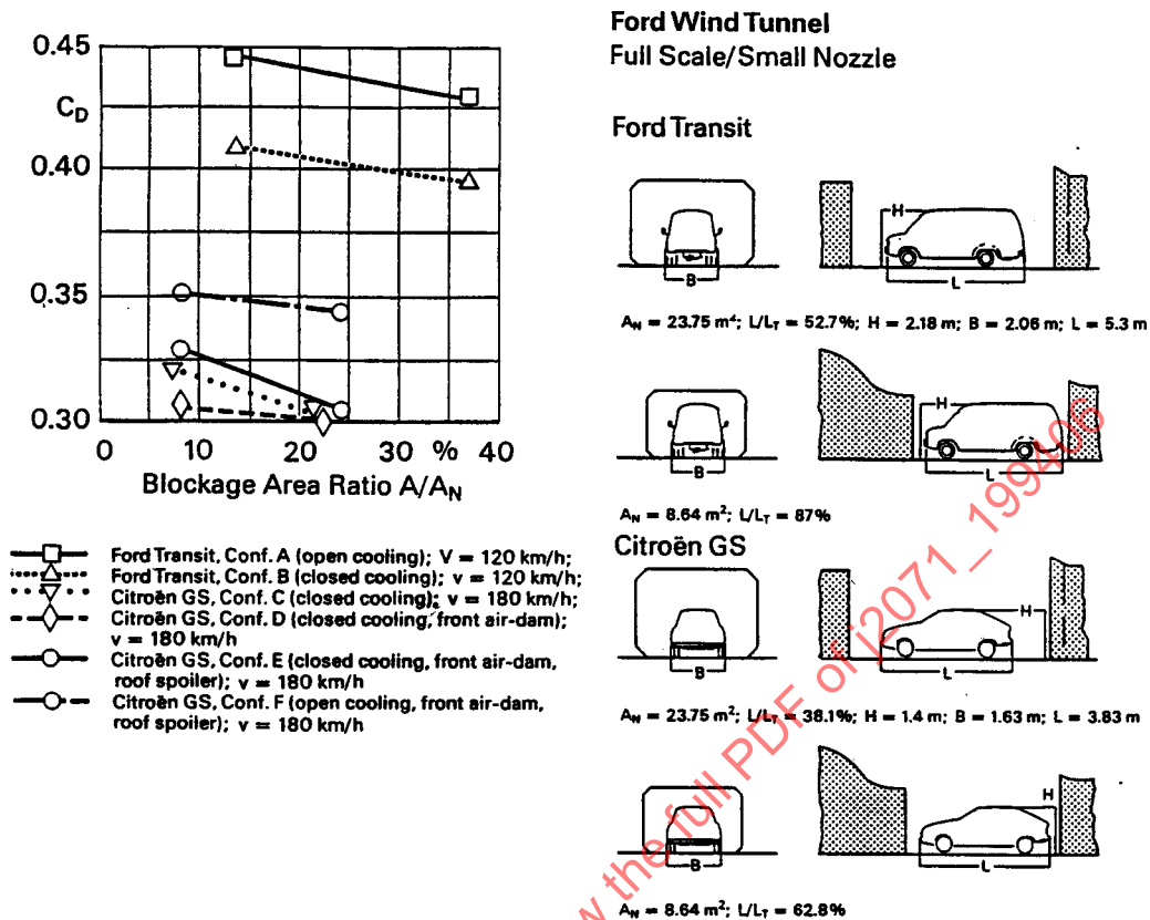
FIGURE 23—DRAG COEFFICIENT OF CARS AS A FUNCTION OF TEST SECTION LAYOUT
