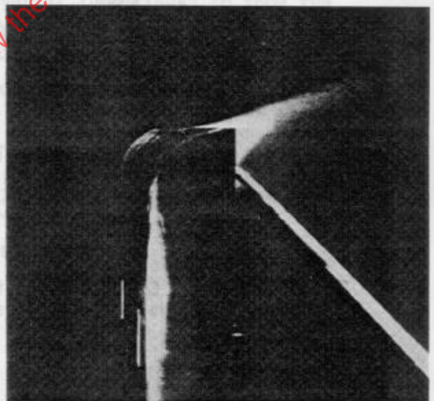
Photo 4 Flat plate with round edge at high Reynolds number Separation at the edge
