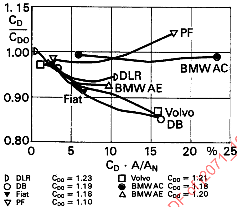
FIGURE 31—RELATIVE DRAG COEFFICIENTS OF SHARP EDGED FLAT PLATES
