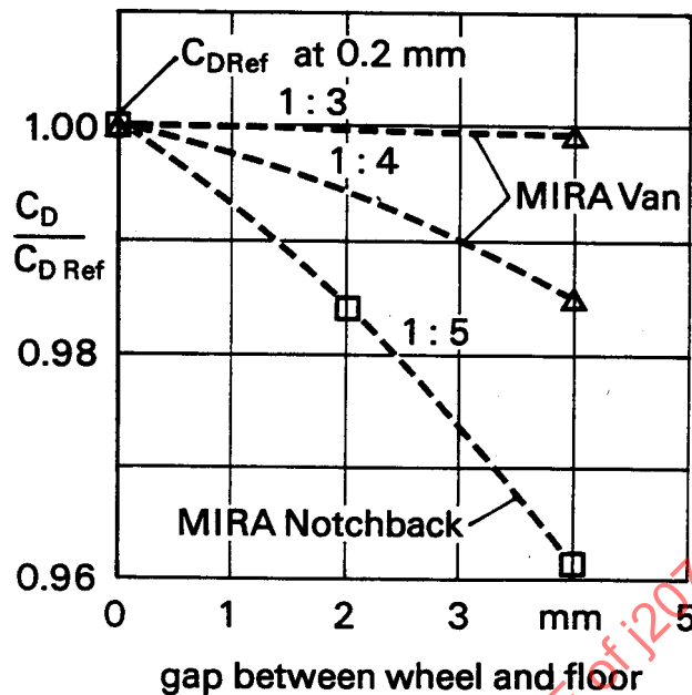
FIGURE 34—GAP INFLUENCE MEASURED IN PORSCHE WIND TUNNEL
