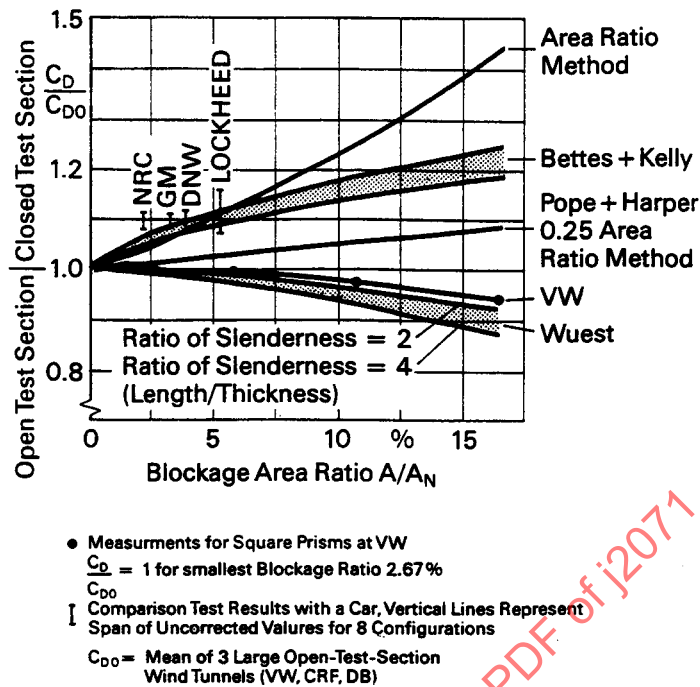
FIGURE 12—BLOCKAGE CORRECTION METHODS VERSUS BLOCKAGE AREA RATIO AFTER REFERENCE 2.1.1 (3)
