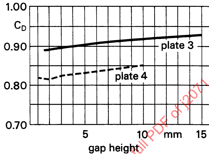
FIGURE 27—EFFECT OF FLAT PLATE DISTANCE FROM THE GROUND
