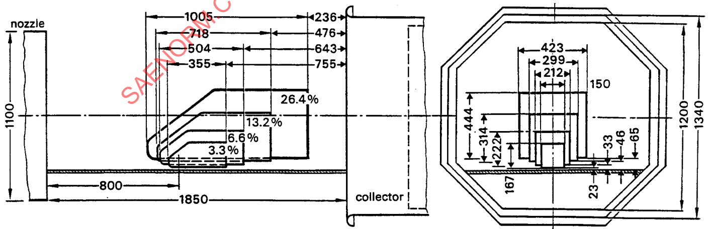
FIGURE 18—MODEL AND TEST SECTION DIMENSIONS AFTER REFERENCE 2.1.2 (13)
