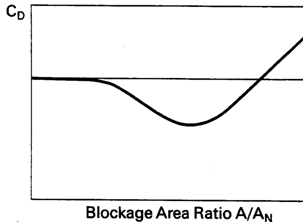
FIGURE 41—QUALITATIVE DRAG CURVE VERSUS BLOCKAGE AREA RATIO CONSIDERING COLLECTOR EFFECTS ONLY
