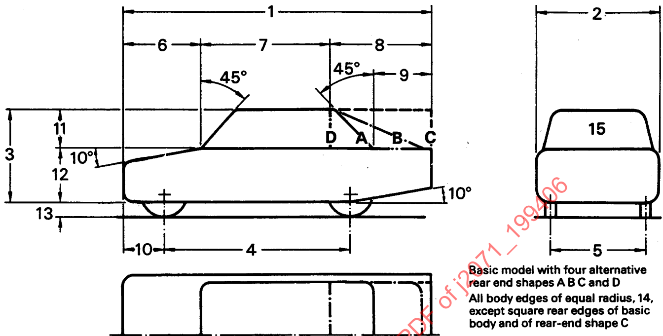
FIGURE 32—DIMENSIONS OF MODELS USED FOR BLOCKAGE STUDY (SEE ALSO TABLE 6)
