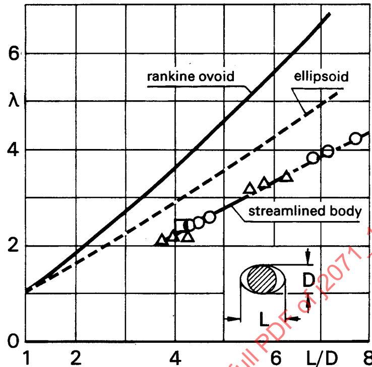
FIGURE 3—MODEL SHAPE FACTOR \lambda AS A FUNCTION OF RELATIVE THICKNESS FOR VARIOUS BODIES OF REVOLUTION AFTER REFERENCE 2.1.2 (4), MODEL PLACED IN CENTERLINE
