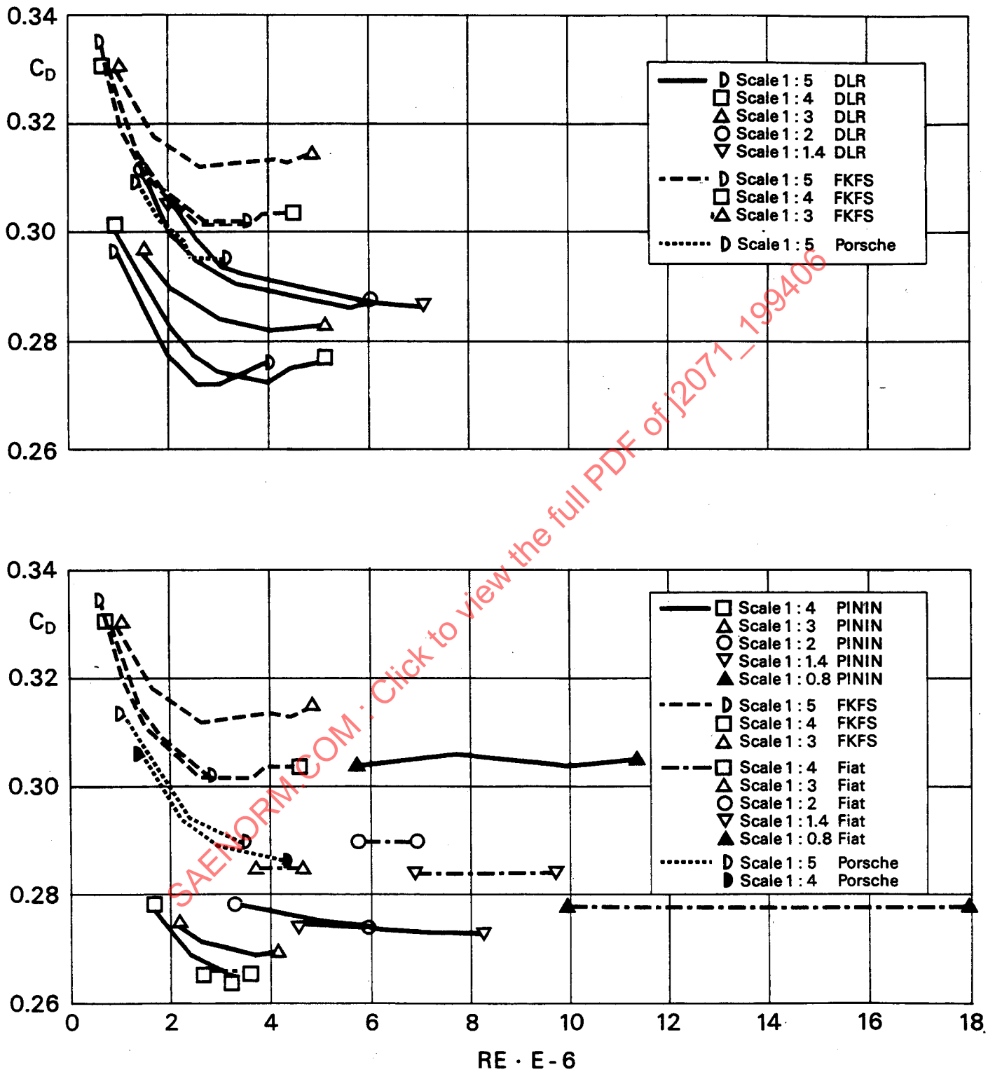
FIGURE 35—DRAG COEFFICIENTS OF MIRA NOTCHBACK MODELS
