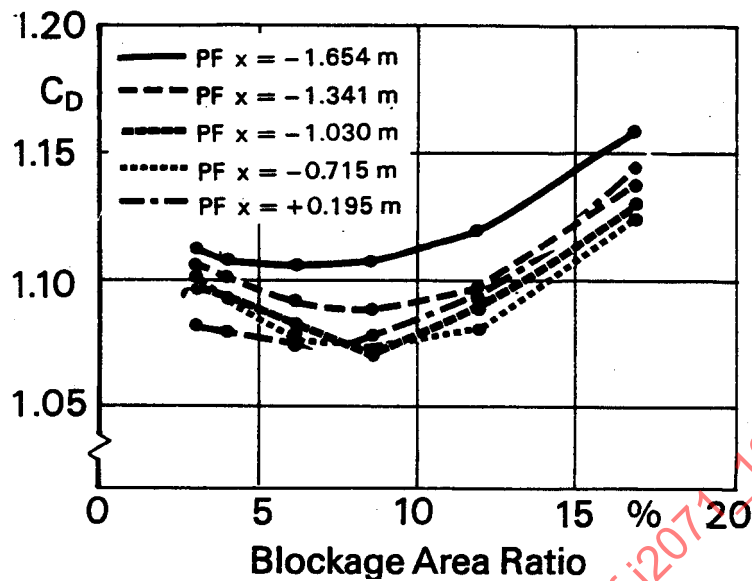
FIGURE 30—DRAG COEFFICIENTS OF SHARP EDGED FLAT PLATES IN PININFARINA WIND TUNNEL AT DIFFERENT POSITIONS (X = DISTANCE FROM BALANCE CENTER)
