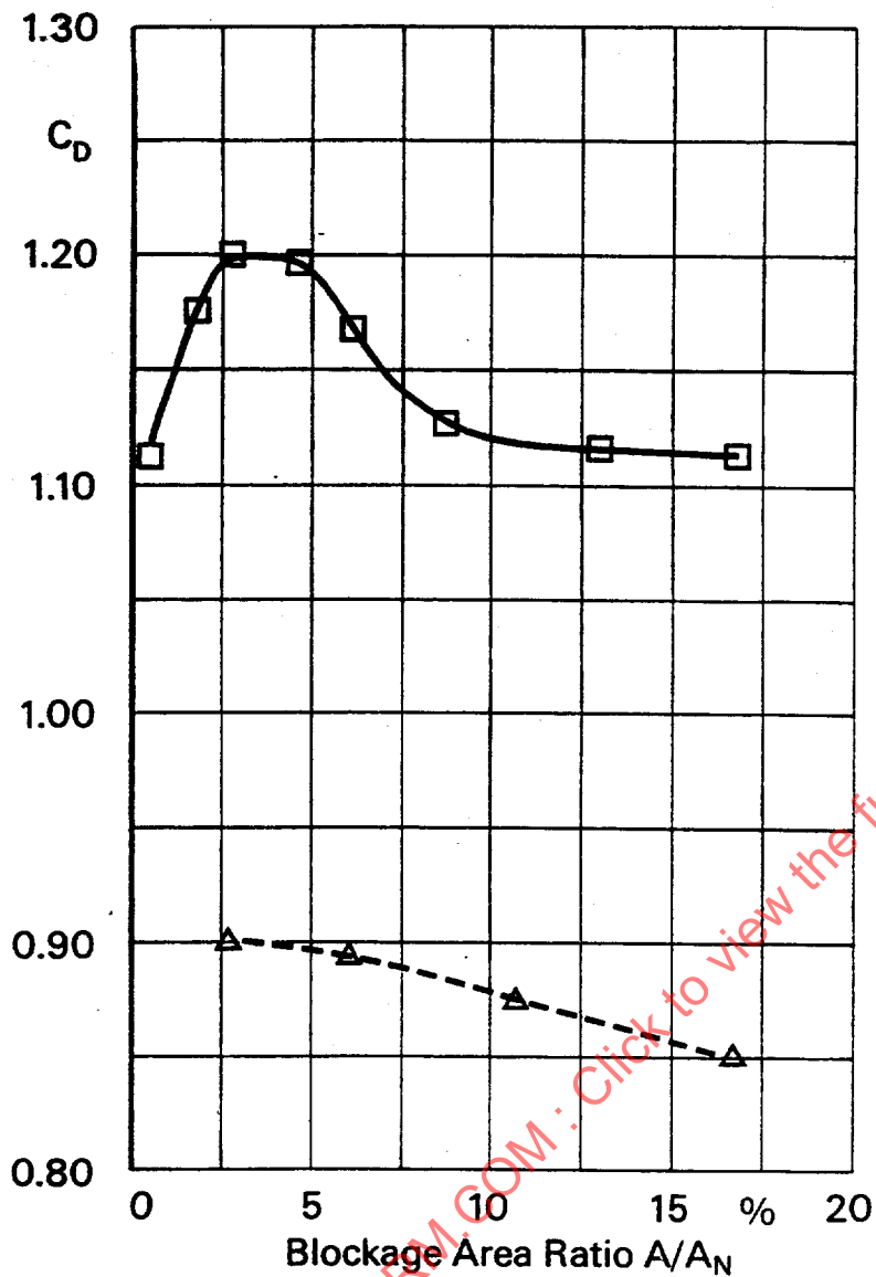
FIGURE 22—DRAG COEFFICIENT OF BLUFF BODIES AS A FUNCTION OF BLOCKAGE AREA RATIO
