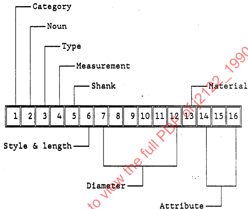
Figure 1 - Numbering System for Drills
