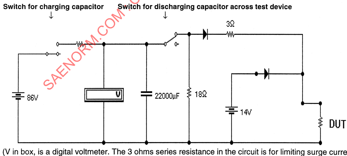
FIGURE 3—EXAMPLE OF A LOAD DUMP TESTING CIRCUIT
