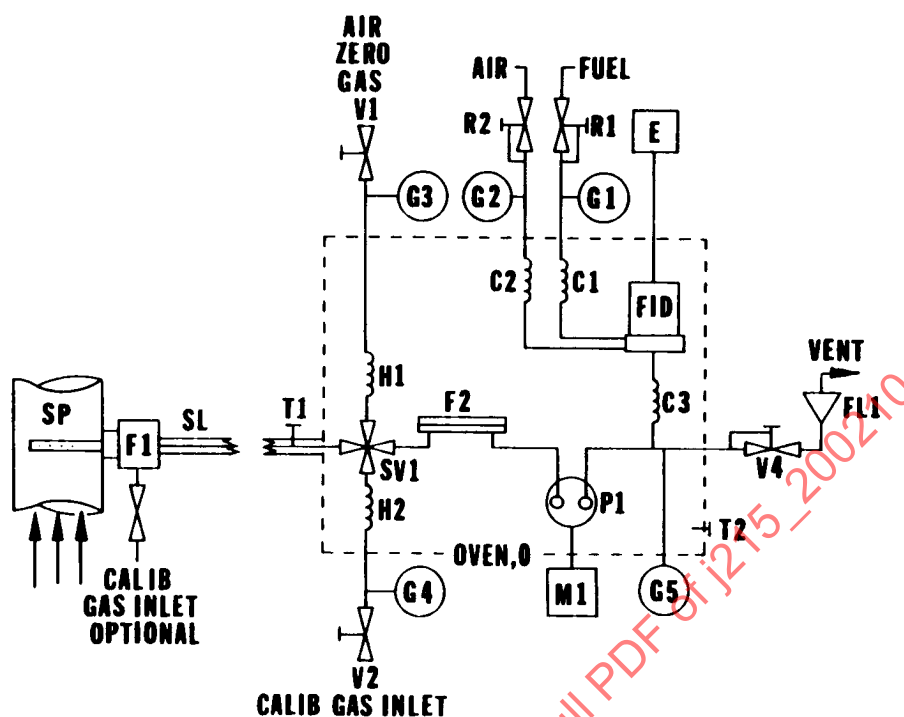
FIGURE 1—CHA POSITIVE PRESSURE BURNER
