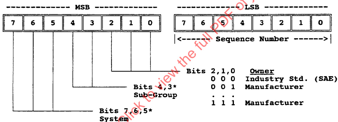
FIGURE 3—PRN STRUCTURE
