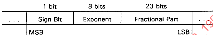
FIGURE 15—SIGNED FLOATING POINT (SCIENTIFIC NOTATION) (SFP) SLOT
