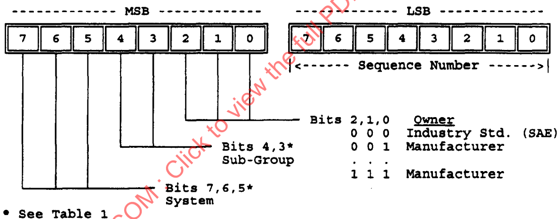
FIGURE 3—PRN STRUCTURE
