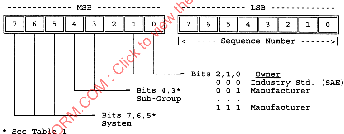
FIGURE 3—PRN STRUCTURE
