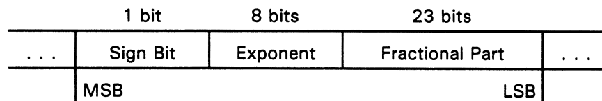
FIGURE 14—SIGNED FLOATING POINT (SCIENTIFIC NOTATION) (SFP) SLOT
