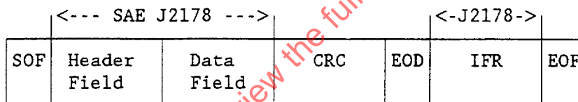
FIGURE 2—SCOPE OF SAE J2178 FOR A SAE J1850 FRAME WITH IN-FRAME RESPONSE (IFR)
