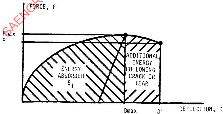
FIGURE 9—LOAD DEFLECTION CURVE—CONTINUING OVERLOAD TEST
