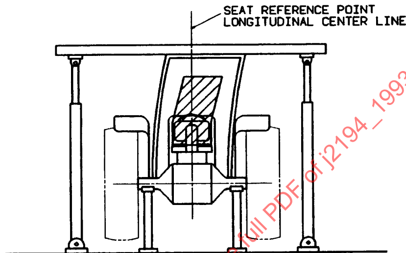
FIGURE 3—TYPICAL LOAD APPLICATION FOR CRUSH TEST
