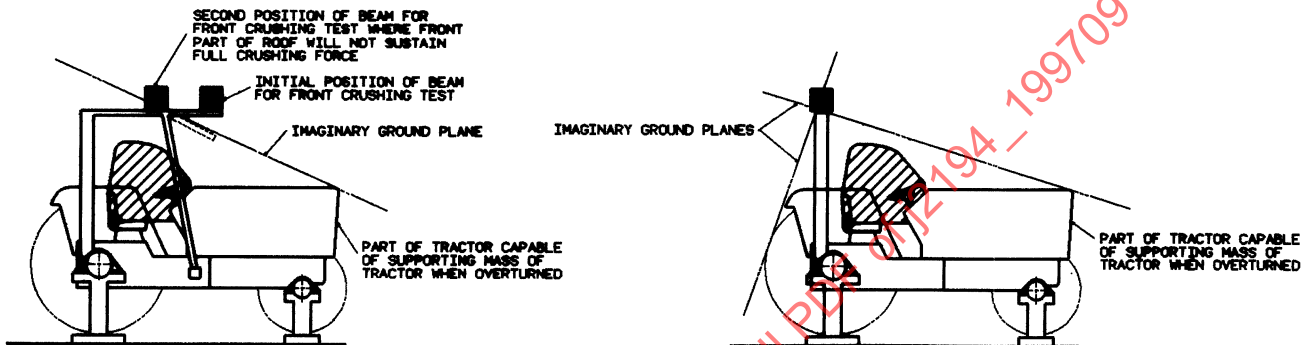
FIGURE 7—FRONT CRUSH
