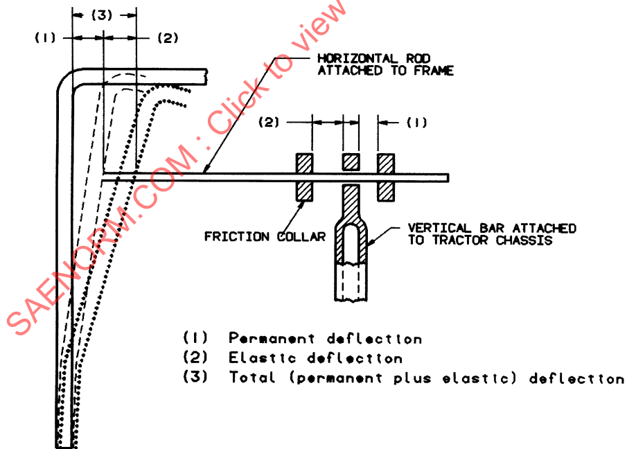
FIGURE 12—TYPICAL METHOD OF MEASURING DEFLECTION
