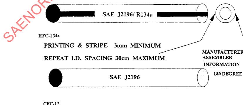
FIGURE 1—SERVICE HOSE
