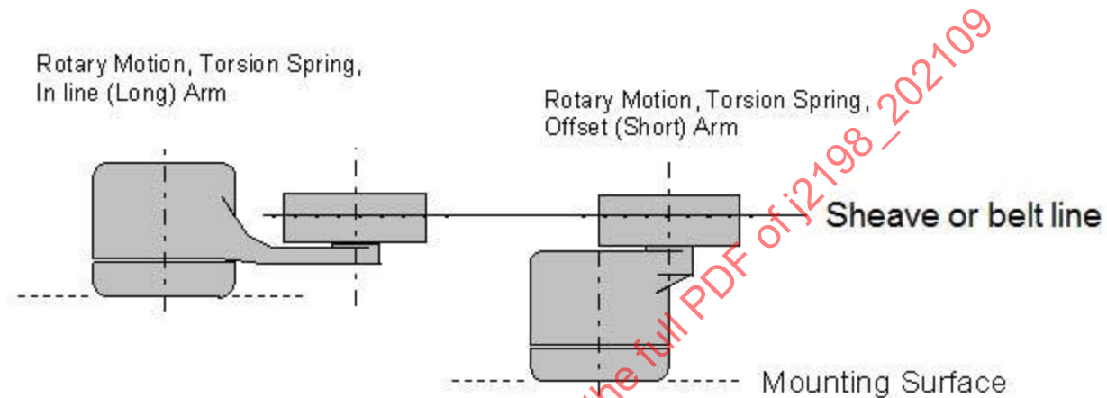
FIGURE 1 - ARM UNDER CONFIGURATION
