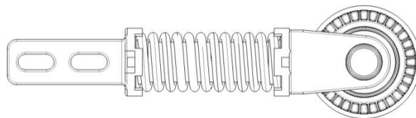
FIGURE 3 – LINEAR MOTION LINEAR SPRING DESIGN
