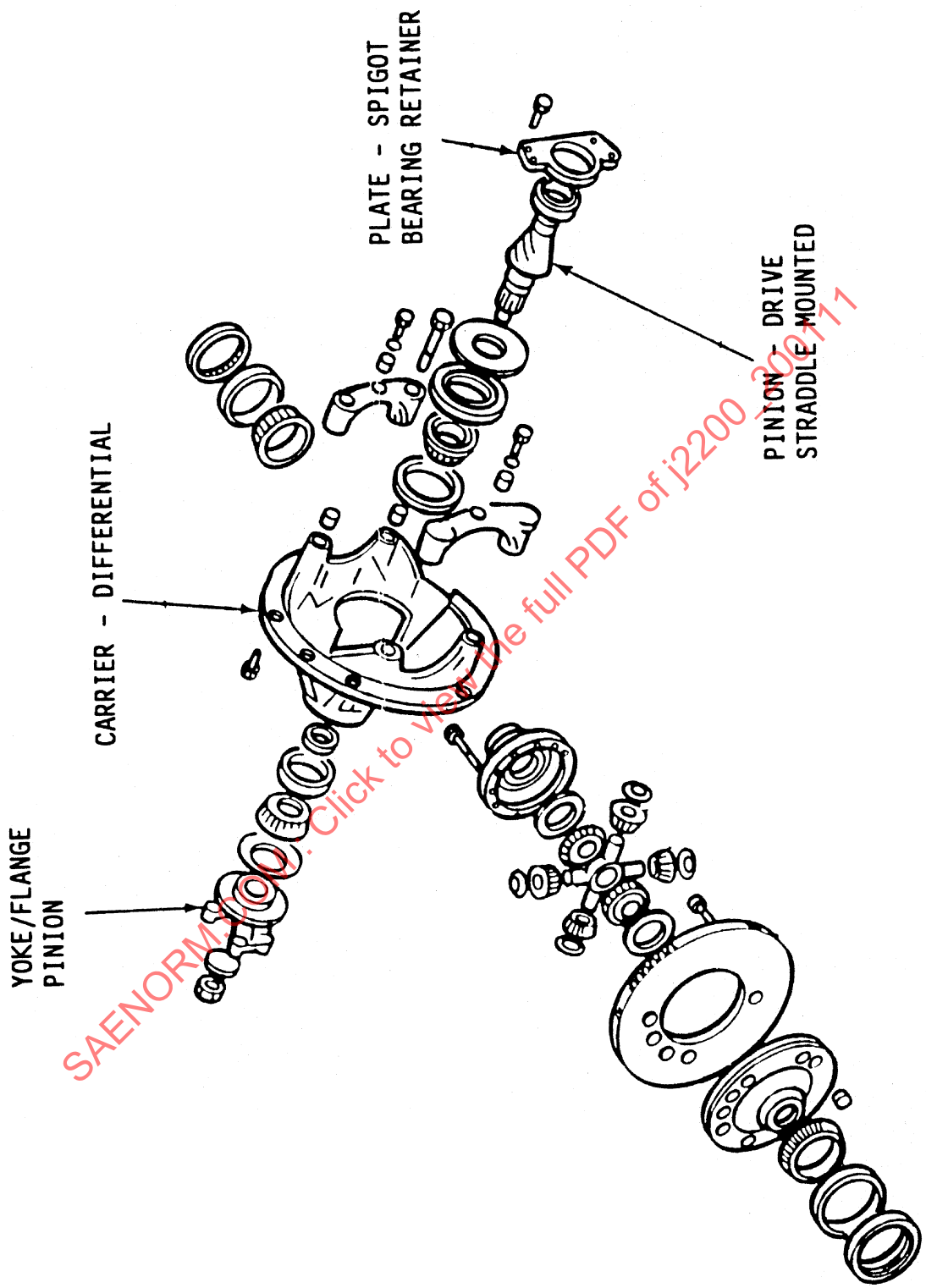
FIGURE 3—STRADDLE MOUNTED PINION
