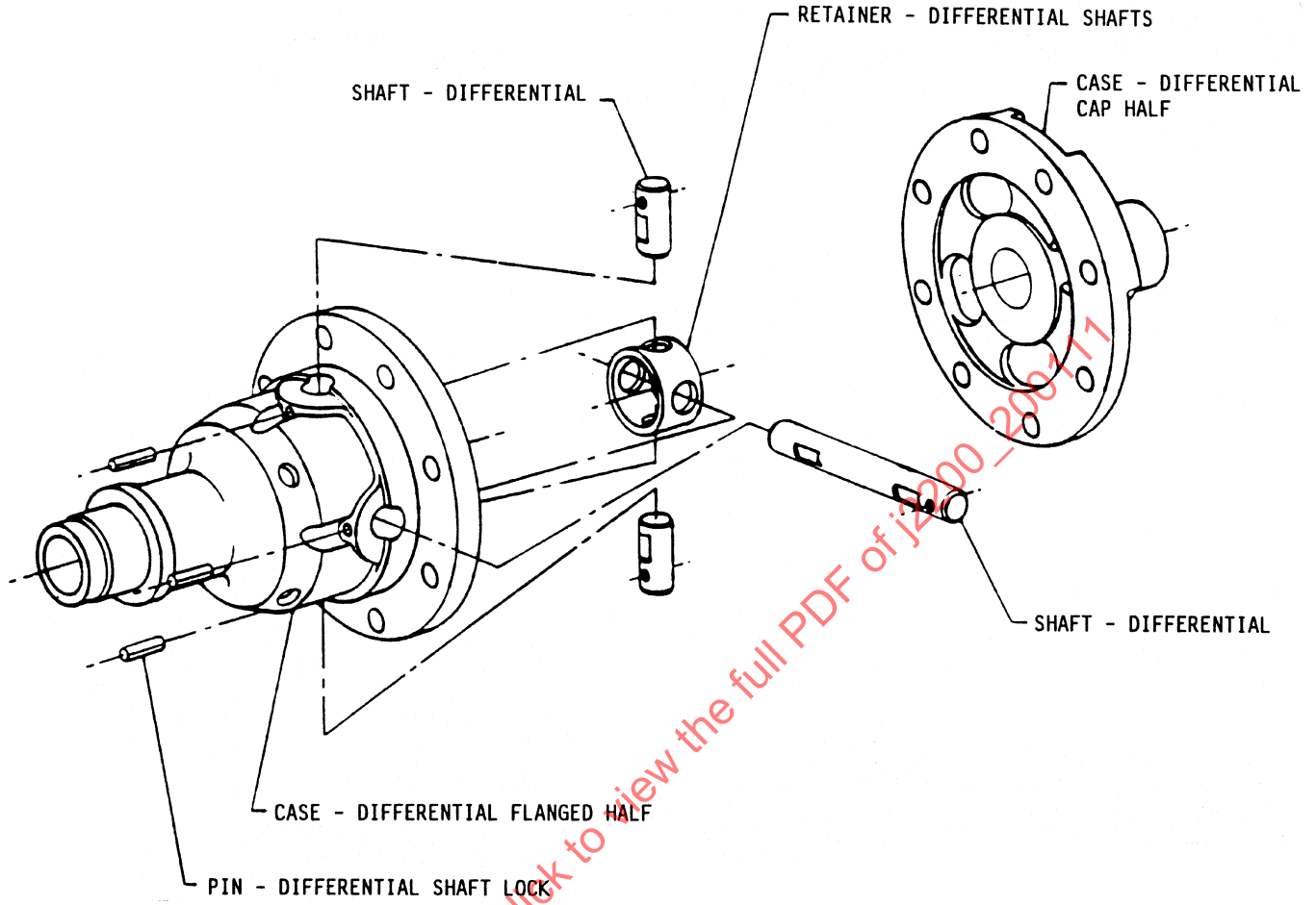
FIGURE 4B—MULTIPLE PINION DIFFERENTIAL (OPTIONAL CONSTRUCTION)
