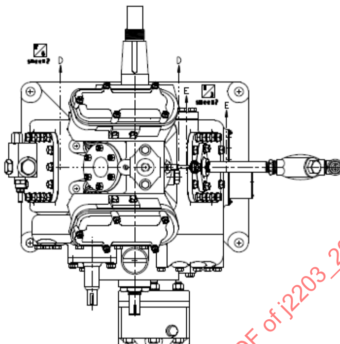
FIGURE 1B - THE 5750 / 16047 ENGINE
