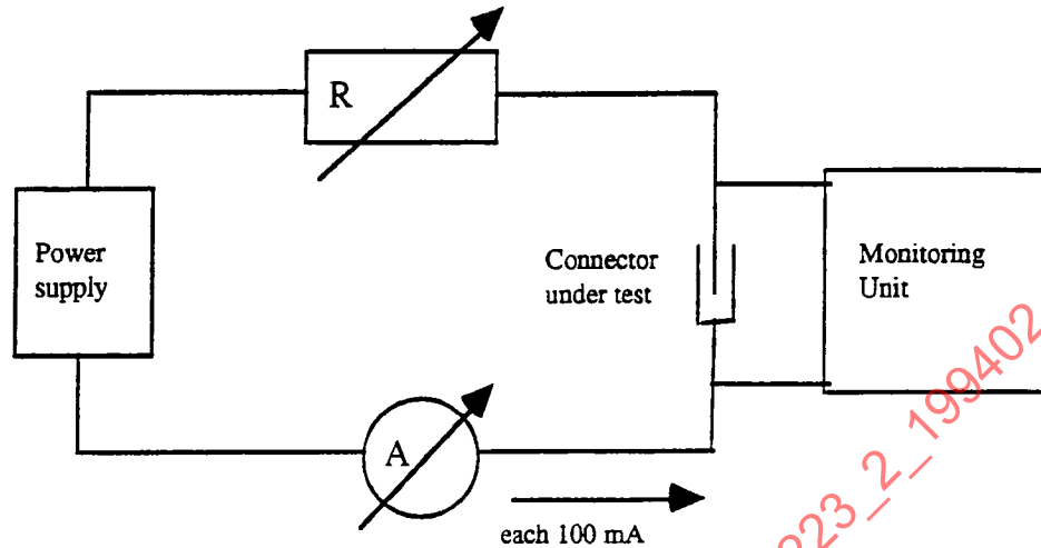
FIGURE 13—CONNECTOR RESISTANCE MONITORING AT VIBRATION TEST
