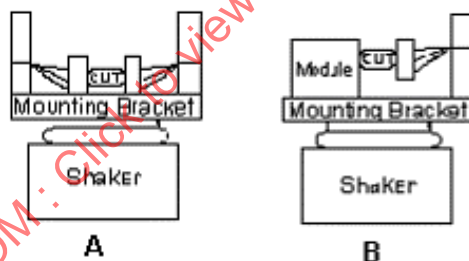
FIGURE 12—MOUNTING POSITIONS
