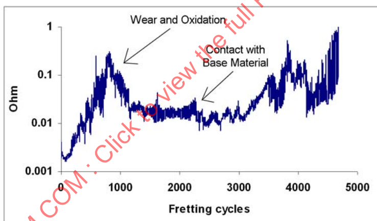
FIGURE 23—EXAMPLE FORCED FRETTING RESISTANCE CURVE OF A TIN CONTACT
