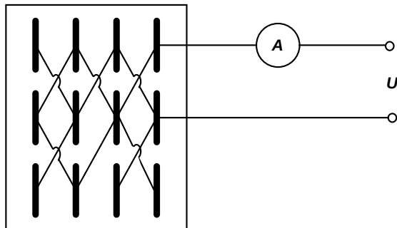
FIGURE 16—METHOD OF CONNECTING LEADS FOR ISOLATION RESISTANCE TEST
