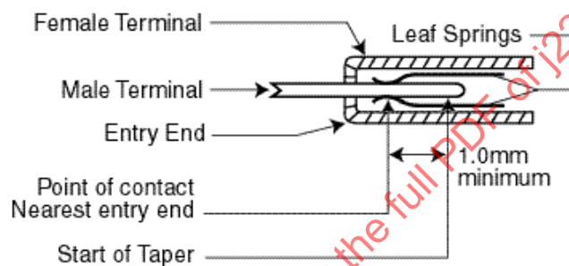
FIGURE 8—TERMINAL INSERTION
