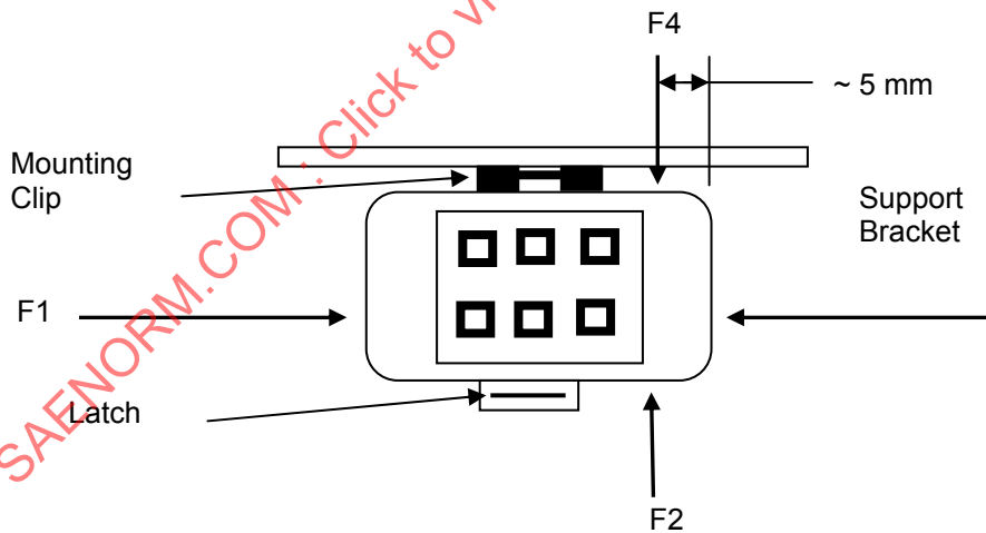
FIGURE 19—TEST SET-UP, END VIEW
