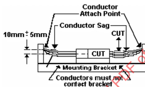
FIGURE 13—TYPICAL CONNECTOR VIBRATION TEST SET-UP
