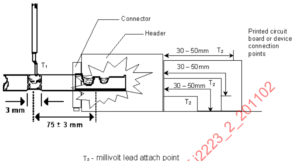
FIGURE 1—METHOD 1 – MILLI-VOLT LEAD ATTACHMENT
