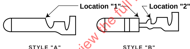
FIGURE 5—TERMINAL DESIGN STYLE
