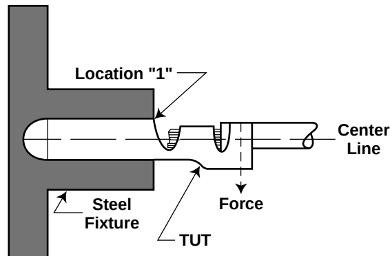
FIGURE 6—TERMINAL BEND TEST
