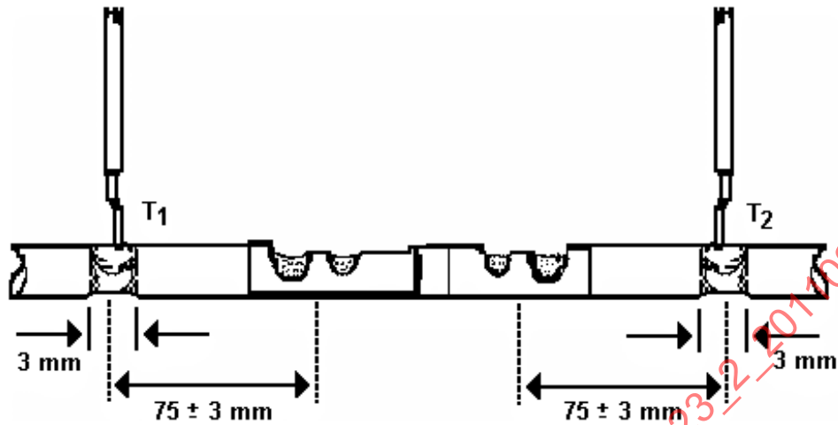
FIGURE 7—CONNECTION RESISTANCE MILLIVOLT LEAD LOCATIONS
