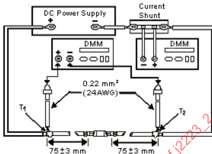
FIGURE 9—CURRENT RESISTANCE TEST SET-UP
