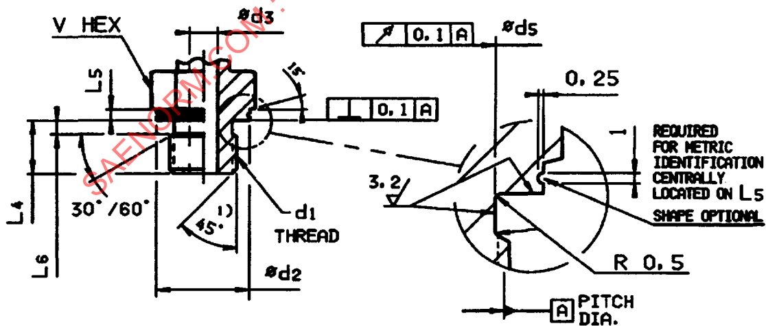
FIGURE 1A—ADJUSTABLE (L SERIES) STUD DETAIL
