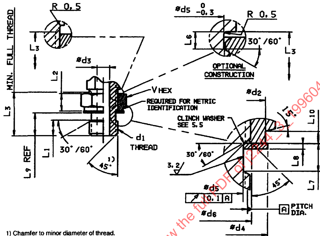
FIGURE 1A—ADJUSTABLE (L SERIES) STUD DETAIL
