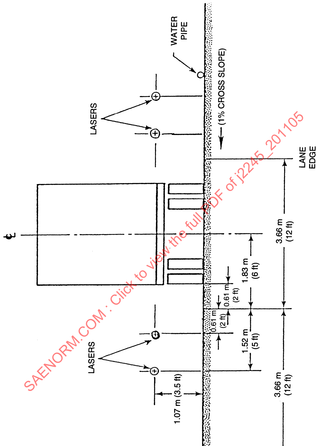
FIGURE 3—LATERAL PLACEMENT OF LASERS WITH RESPECT TO TEST VEHICLE
