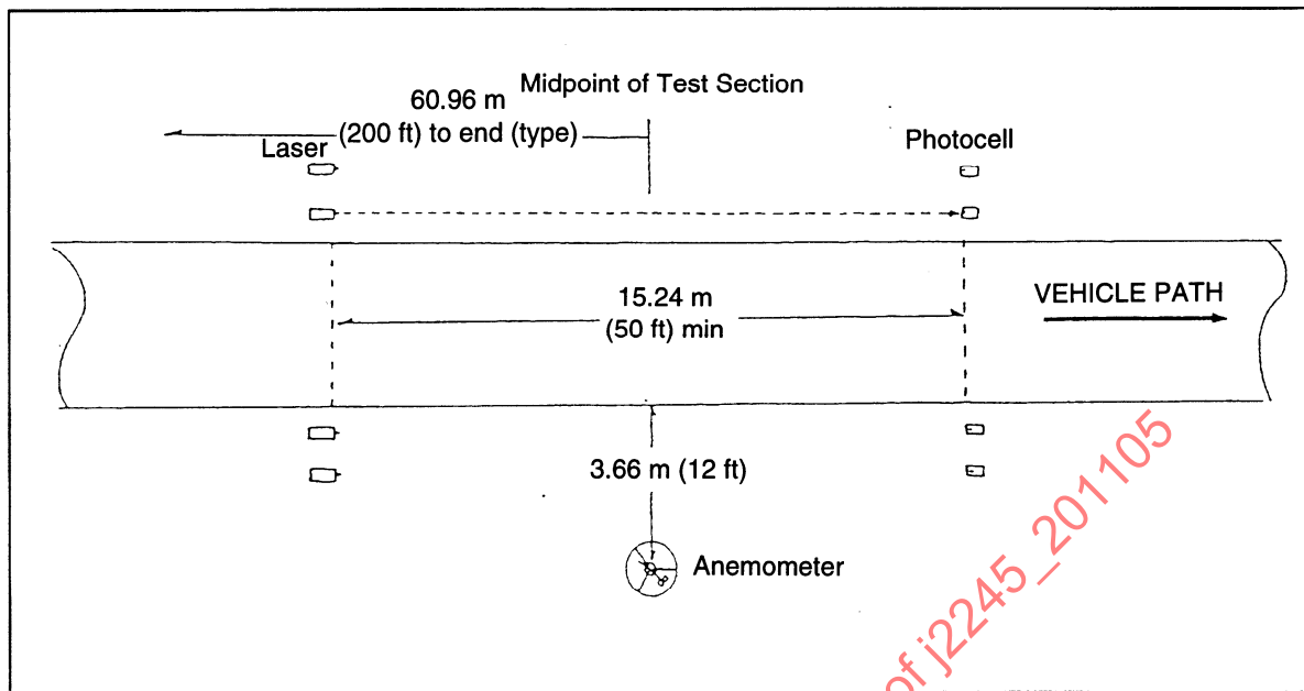
FIGURE 4—ANEMOMETER SET LOCATION
