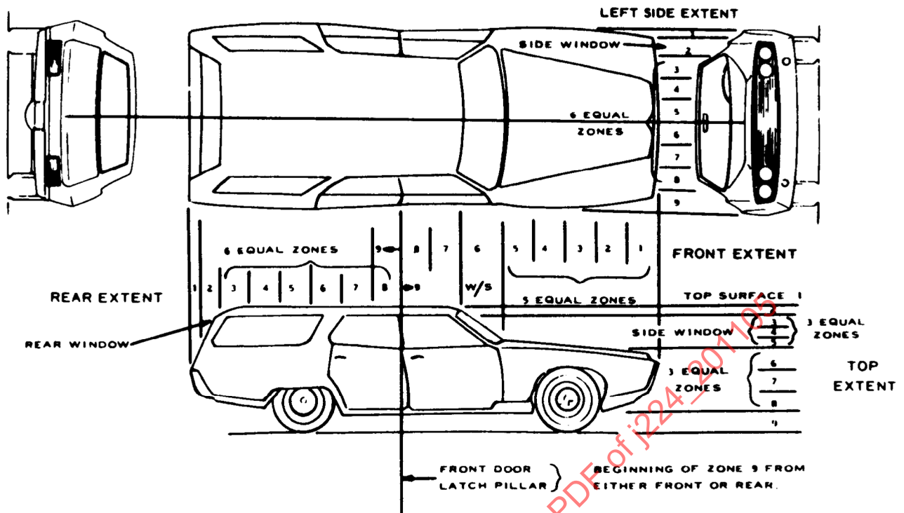
FIGURE 7—DEFORMATION EXTENT ZONES (FOR STATION WAGONS)
