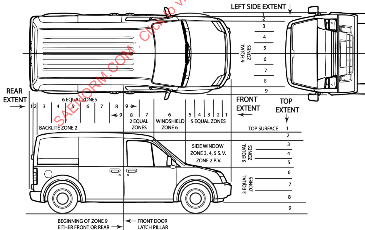
Figure 8 - Deformation extent zones (for vans)
