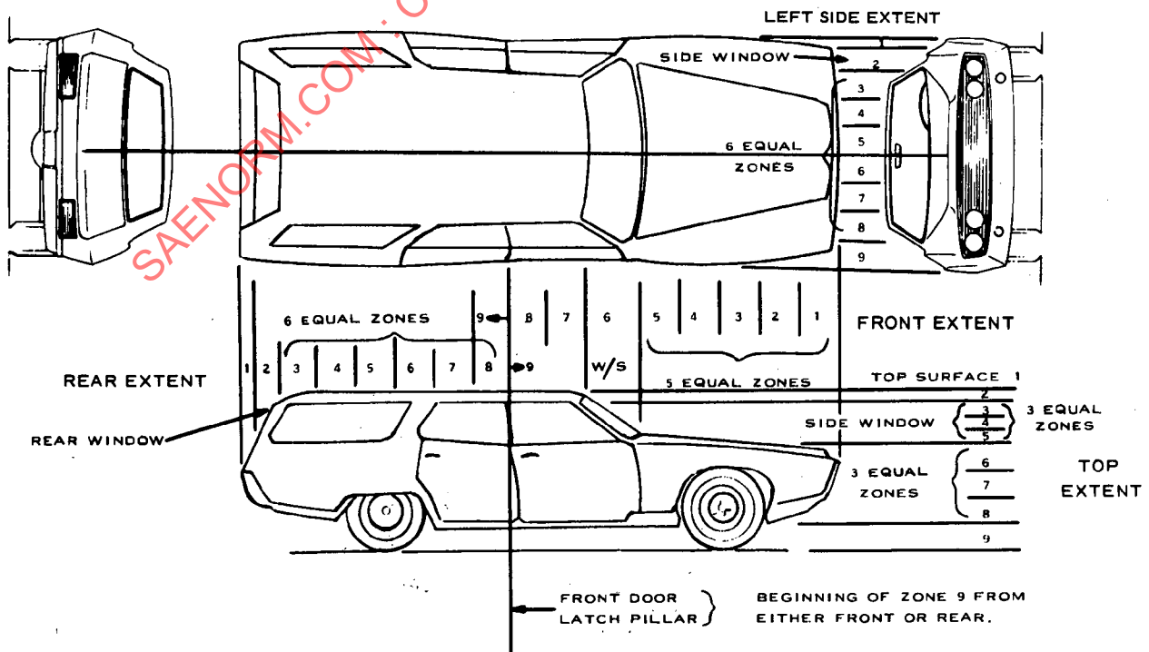
FIG. 8—DEFORMATION EXTENT ZONES (FOR STATION WAGONS)
