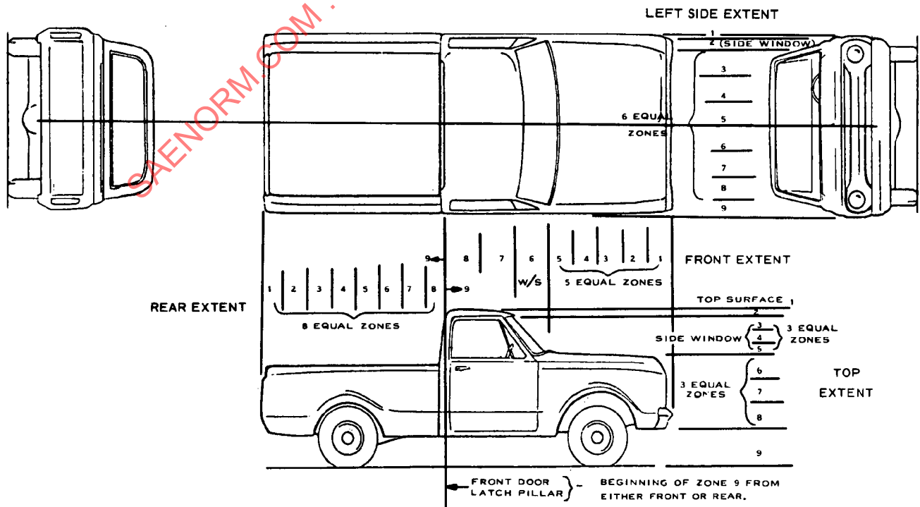
FIG. 10-DEFORMATION EXTENT ZONES (FOR PICKUP TRUCKS)
