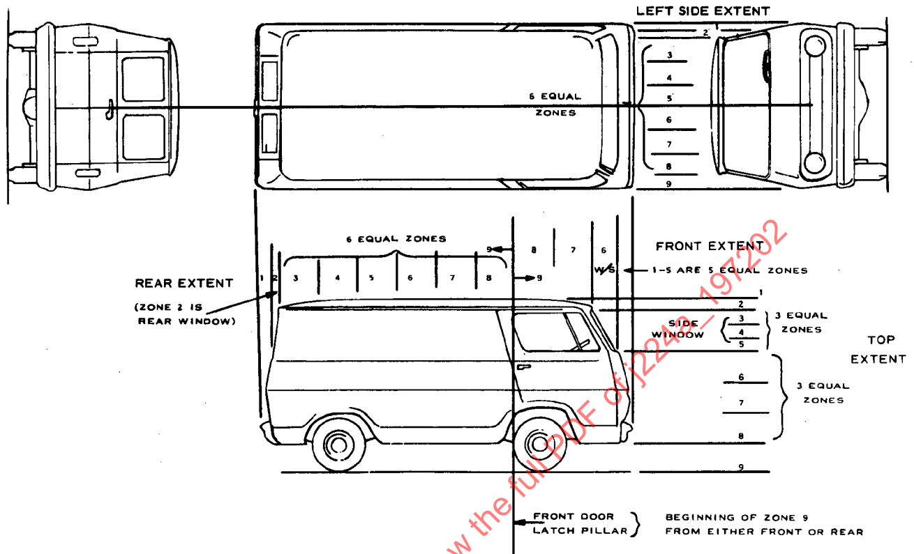
FIG. 9-DEFORMATION EXTENT ZONES (FOR VANS)
